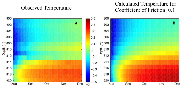
Fig. 7. Left: Observed residual temperature for the Tohoku-oki earthquake as a function of depth (vertical) and time (horizontal). Right: Calculated temperatures assuming a coefficient of friction of 0.1. From Fulton et al., 2013.
