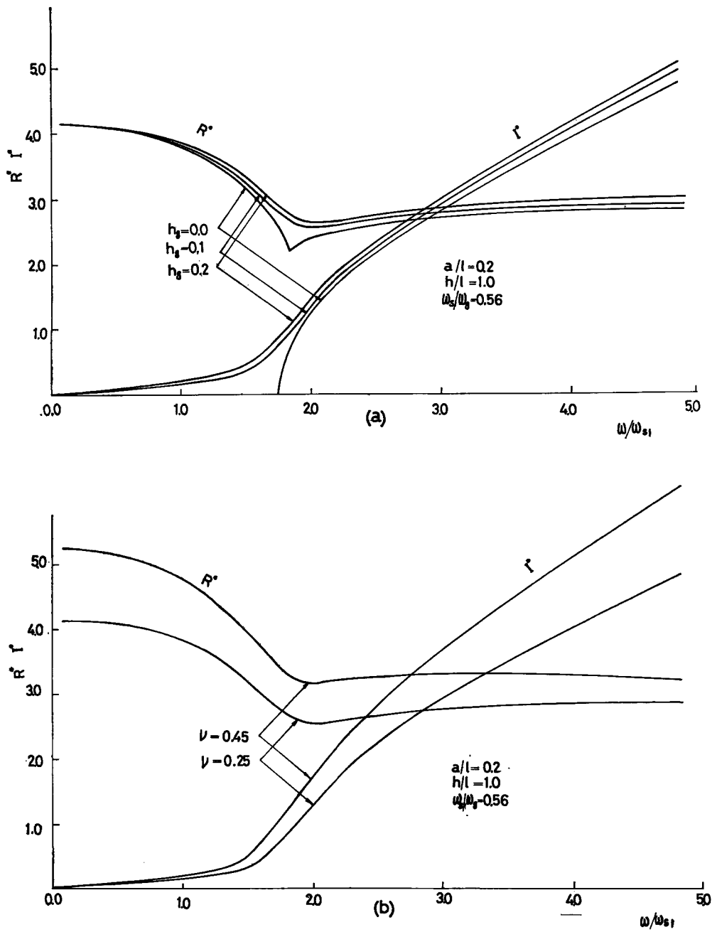
Fig. 10 Resonance curves of R^* , and I^* .
