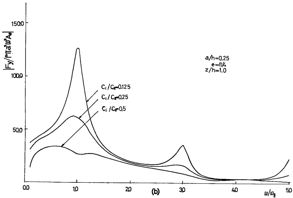
Fig. 5 Resonance curves of earth pressure.
