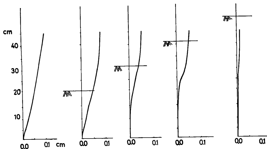
Fig. 17 Deflection curves of structure.
