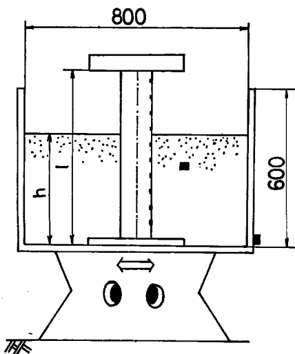
Fig. 13 Experimental devices.
