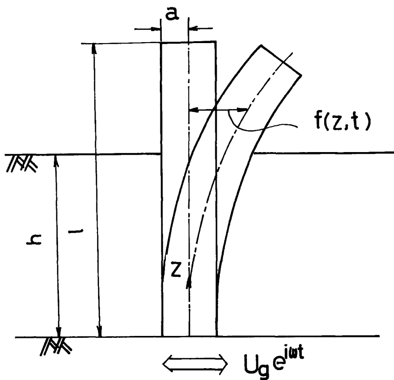
Fig. 7 Model of system.
