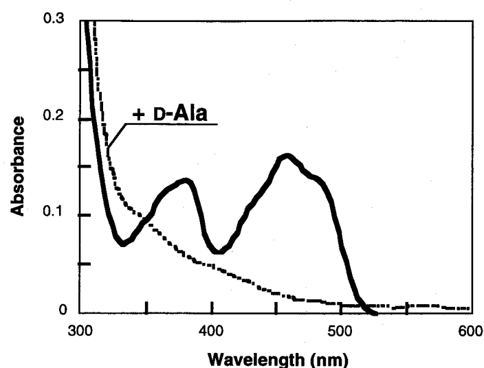
Fig. 3-3. Absorption spectra of C. boidinii DAO. Solid line: purified DAO (2.0 mg/ml) in 0.1 M KPB, pH 8.0; broken line: purified DAO (2.0 mg/ml) incubated with 0.5 M D-alanine in 0.1 M KPB, pH 8.0, at 30°C for 30 min.
