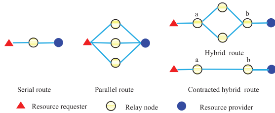
Fig. 4 Availability of routes.
