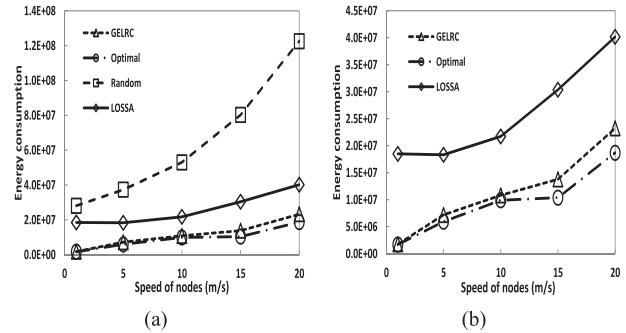
Fig. 5 Energy consumed by different methods.
