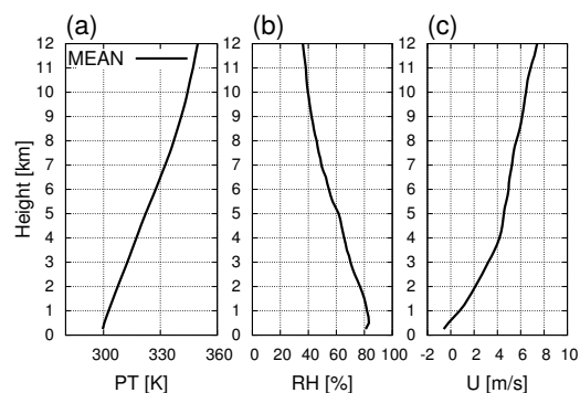
Fig. 1 Initial condition of vertical profiles of (a) temperature [K], (b) relative humidity [%], and (c) zonal wind [ \text{m s}^{-1} ] whose properties are averaged in Pacific region during July-to-August in Unuma and Takemi (2014).
