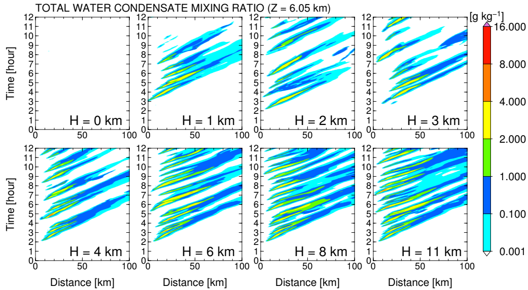
Fig. 3 The horizontal-time variation of total water- and ice-phase mixing ratio [ \text{g kg}^{-1} ] at 6.05 km during the simulations.
