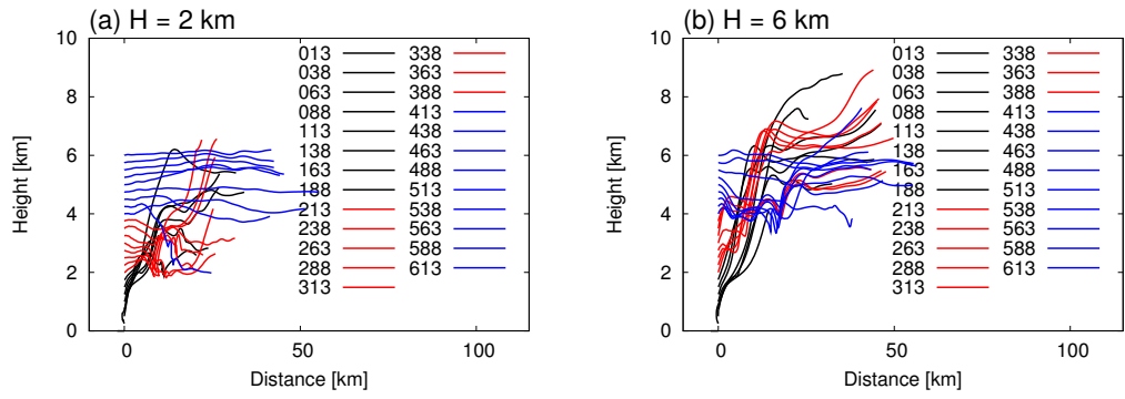
Fig. 5 Forward trajectories for the experiments of (a) H = 2 and (b) 6 km. The legends indicate parcel number of these experiments. Black, red, blue solid lines show the parcel paths which is lifted from within 0–2 km, 2–4 km, and 4–6 km, respectively.
