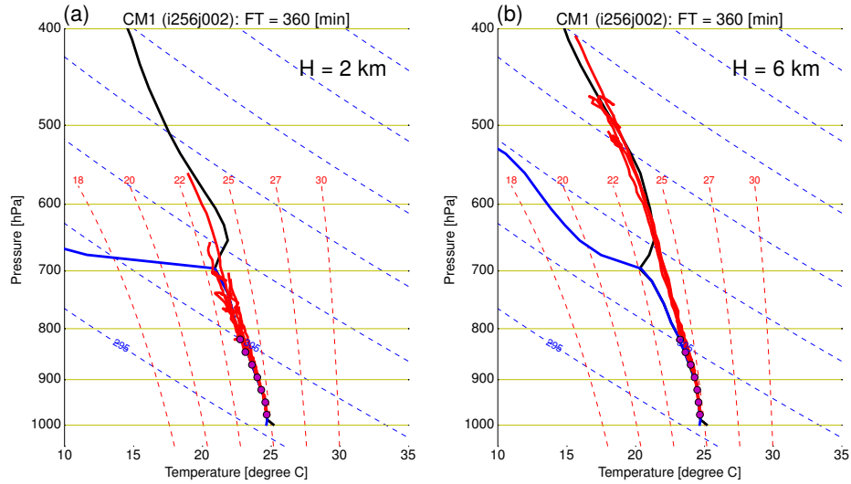
Fig. 7 The skew-T diagrams for (a) H = 2 km and (b) 6 km cases with the parcel paths (red solid line) which is lifted from different heights (indicated by purple circle).
