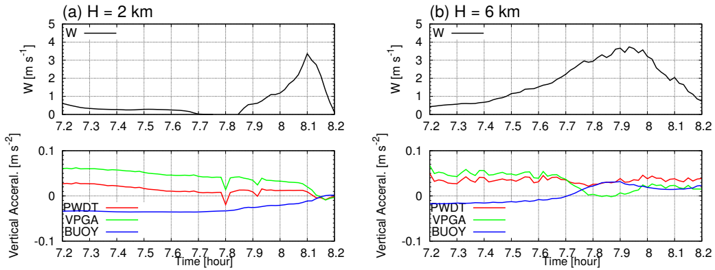
Fig. 6 Time series of the vertical velocities and that of the momentum budget analyses along the trajectory of #113 for (a) H = 2 and (b) 6 km cases.
