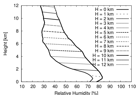
Fig. 2 The vertical profiles of relative humidity for the sensitivity experiments of moisture. Each profiles having moist layer depth (H) are also indicated.
