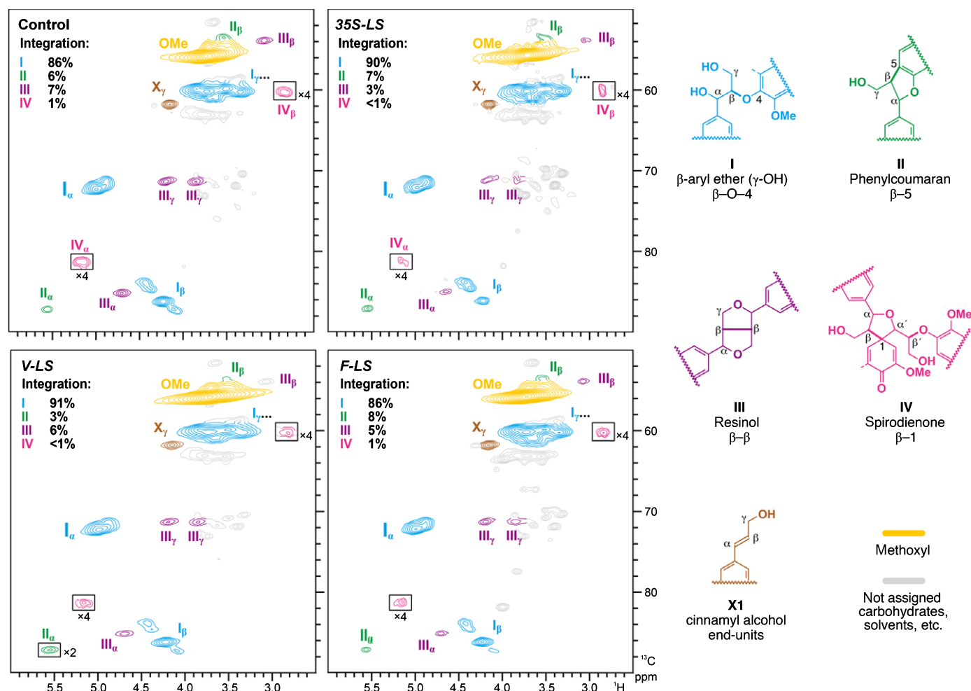
Fig. 5 Aliphatic subregions of short range ^1\text{H} – ^{13}\text{C} correlation (HSQC) NMR spectra of lignin samples prepared from the control, constitutive (35S-LS), vessel-specific (V-LS) and fibre-specific (F-LS) overexpression of LTF1 AA in Populus are shown. Volume integrals are given for the major lignin side-chain structures that are colour-coded to match their assignments in the spectra. The percentages noted in each spectrum are integrals expressed relative to the total I, II, III and IV side-chain structures. Boxes labelled \times 2 and \times 4 indicate regions that are vertically scaled up by two-fold and four-fold, respectively.
