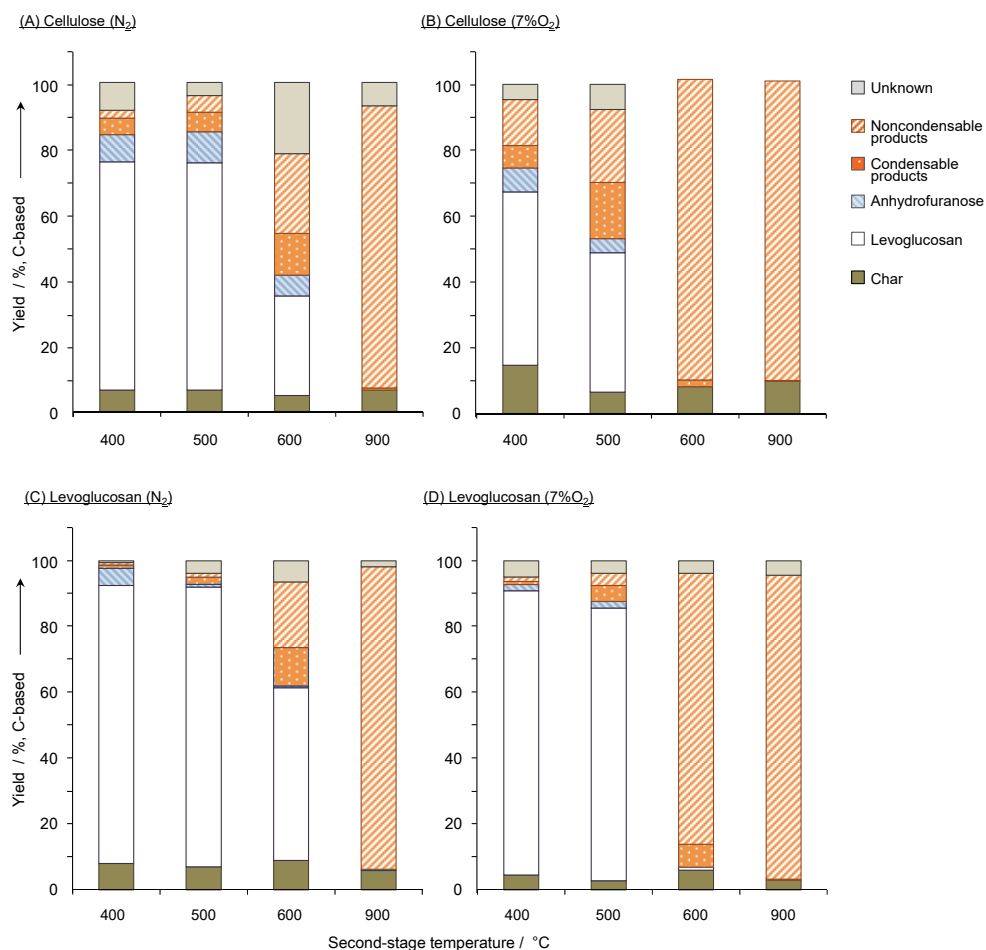
Figure 3. Product compositions from the pyrolyses of cellulose (A, B), levoglucosan (C, D) at the second-stage temperatures of 400, 500, 600, 900 °C under N_2 , 7% O_2/N_2 flow (primary pyrolyzer: 500 °C).
