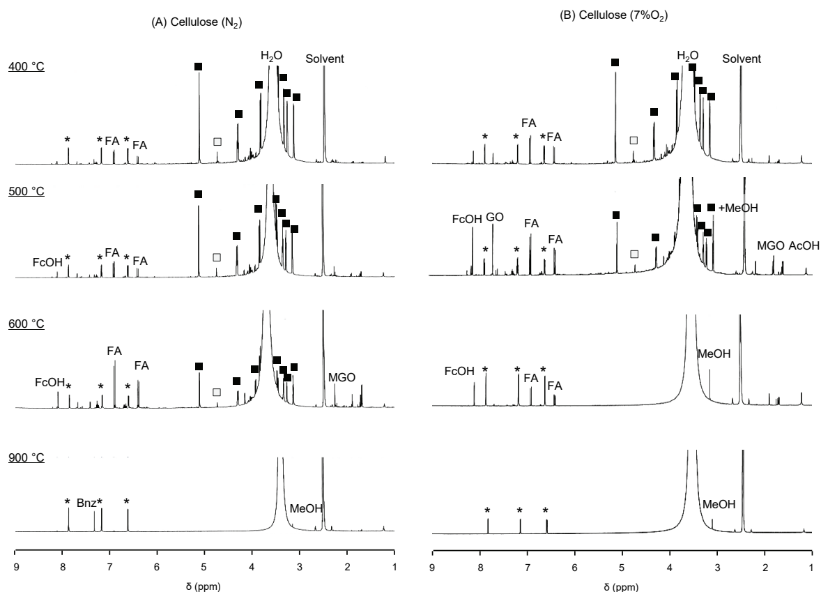
Figure 2. 1 H-NMR spectra of the condensable products recovered in the gas-wash bottle (DMSO- d 6 ) including the oximation reagents during the pyrolysis of cellulose at the second-stage temperatures of 400, 500, 600, 900 °C under N 2 , 7% O 2 /N 2 flow (primary pyrolyzer: 500 °C); ■: levoglucosan, □: 1,6-anhydro-β-D-glucofuranose, *: internal standard (2-furancarboxylic acid), FA: formaldehyde, FcOH: formic acid, GO: glyoxal, MeOH: methanol, MGO: methylglyoxal, AcOH: acetic acid, Bzn: benzene.
