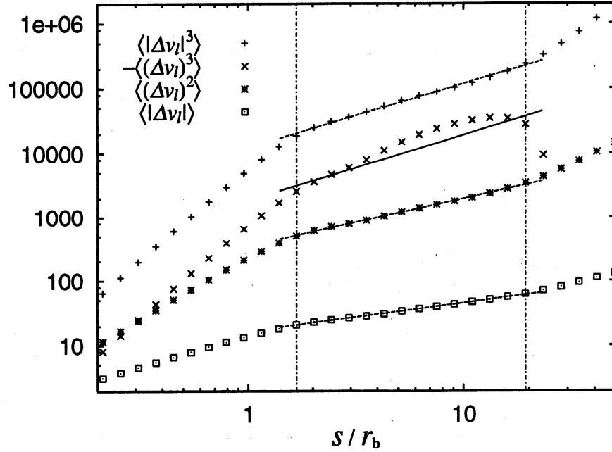
FIG. 4. The first-, second- and third-order structure functions for R_\lambda = 2000 . The region between the dotted lines is regarded as inertial range. Solid line is given by the Kolmogorov's four-fifths law (3) with \varepsilon = (\pi R_0^2)^{-1} \int_0^\infty dR_\Gamma \int_0^{R_0} \varepsilon_{\text{loc}}(R_\Gamma, r) P(R_\Gamma) 2\pi r dr , and dashed lines are the least-log-squares fits within the inertial range.
