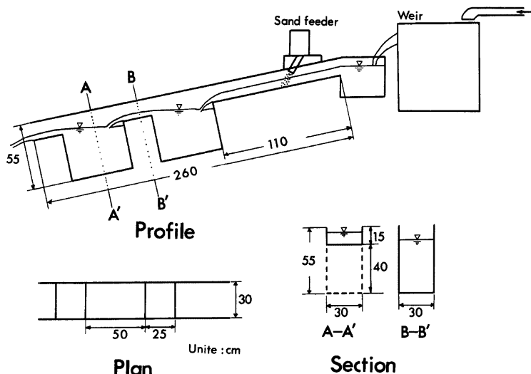
Fig. 20. Experimental flume.
