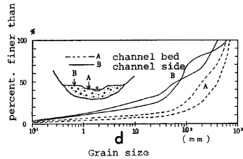
Fig. 5. Grain-size distribution curves.
