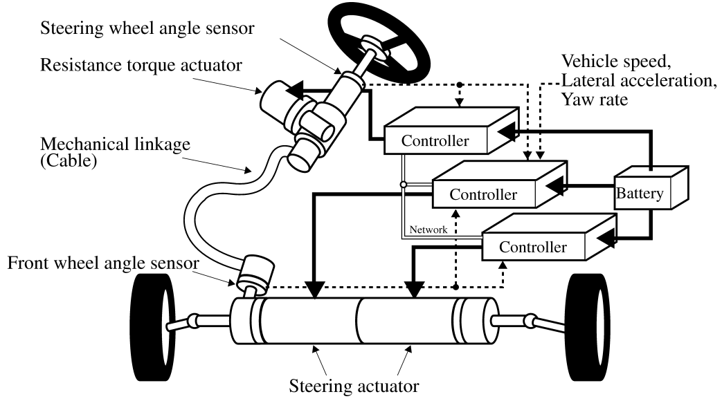
Figure 6: Diversified backup (mechanical and electrical)
