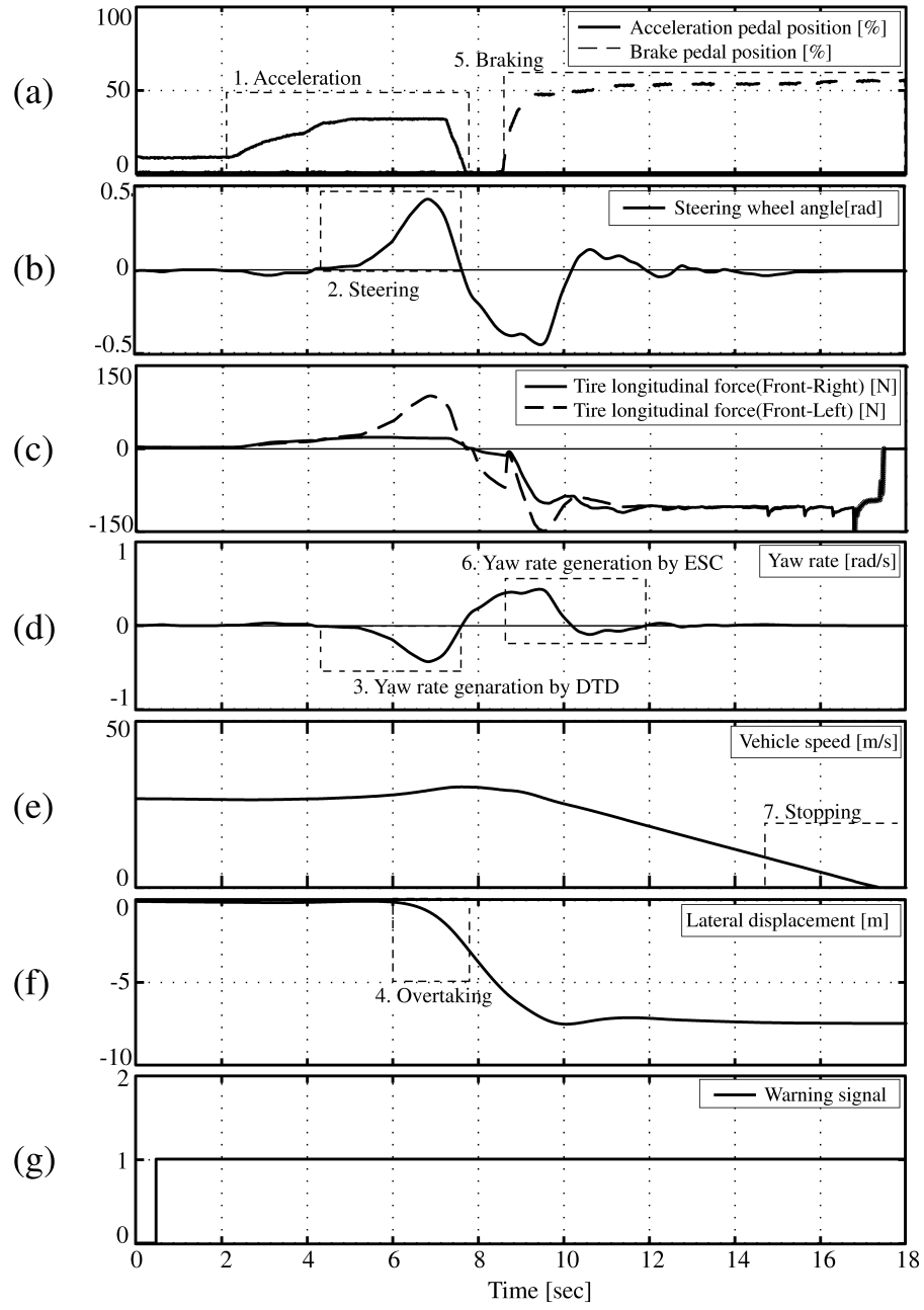
Figure 13: Simulation test result
