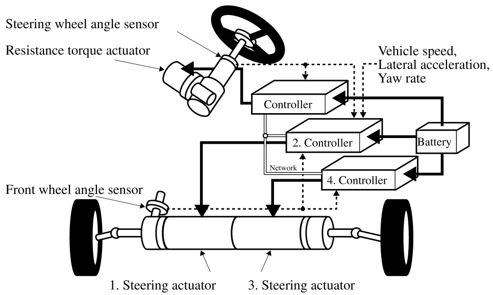
Figure 5: Electric motor backup design
