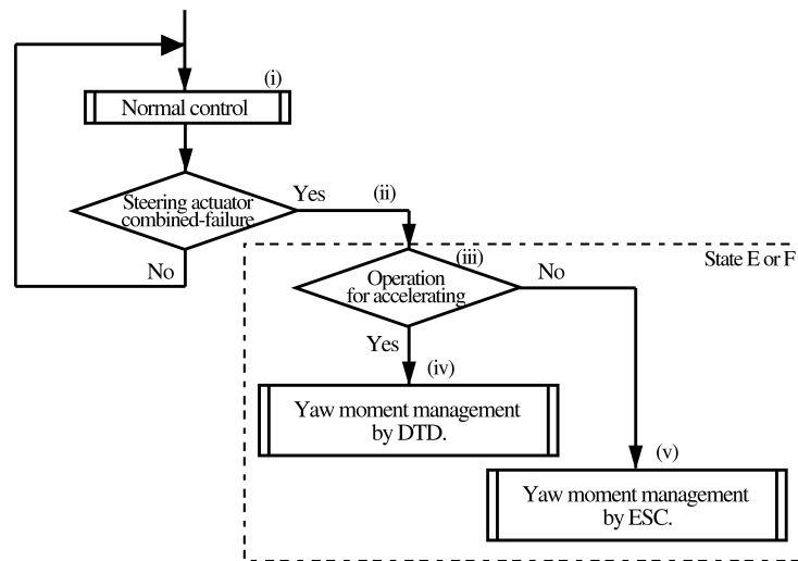
Figure 11: Activation of suitable control mode
