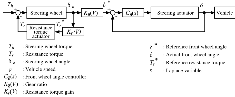
Figure 2: Basic control diagram
