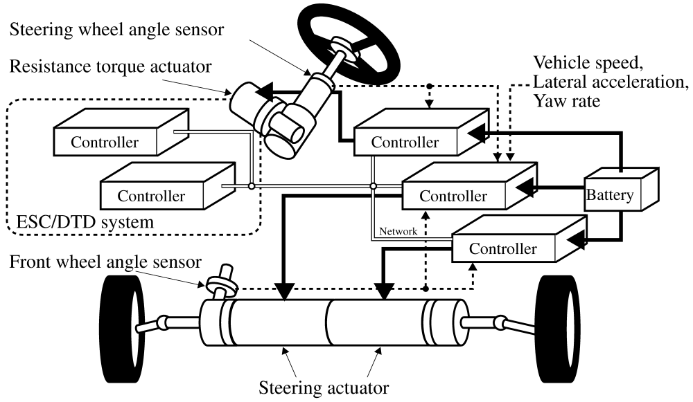
Figure 8: Integrated control architecture
