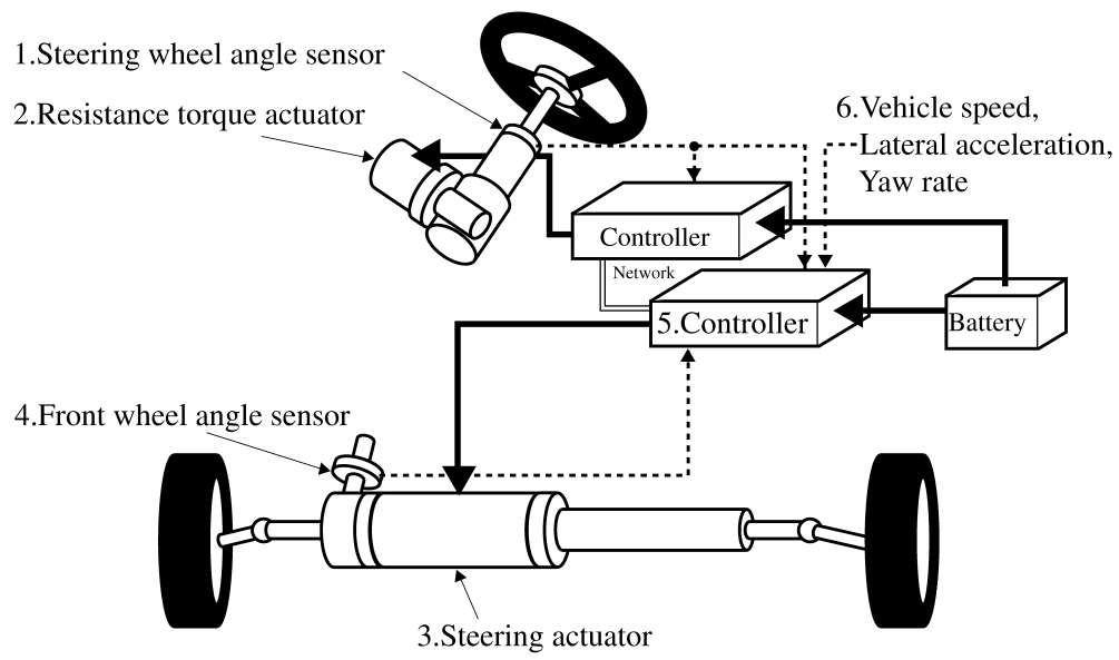
Figure 1: Baseline SBW system structure
