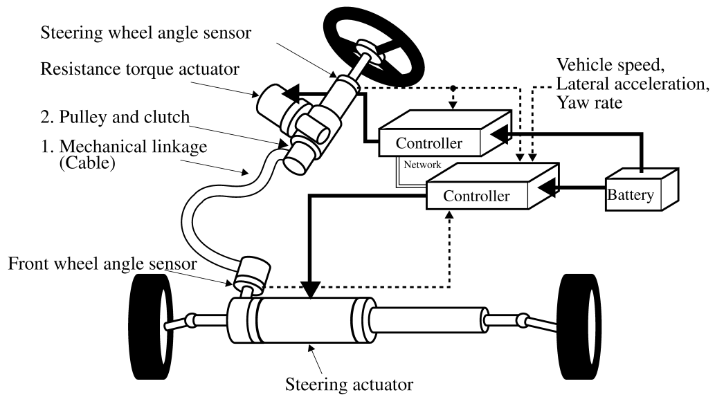
Figure 4: Mechanical cable wire backup design
