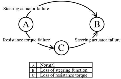
Figure 3: State transition of baseline SBW
