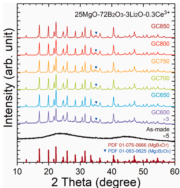
Fig. 3. XRD patterns of the prepared samples with the reference data of crystalline MgB 4 O 7 (PDF #01-076-0666).
