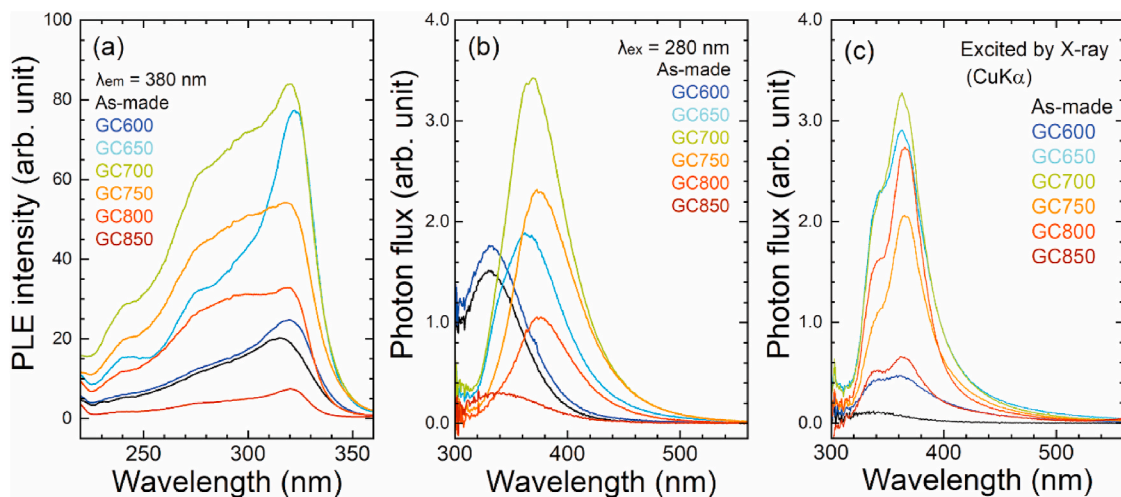
Fig. 6. (a) PLE spectra of all the samples, monitoring \text{Ce}^{3+} emission at 380 nm. (b) PL spectra of all the samples under UV ( \lambda_{\text{ex}} = 280 nm) illumination. (c) RL spectra of all the samples under Cu K \alpha characteristic X-ray illumination.
