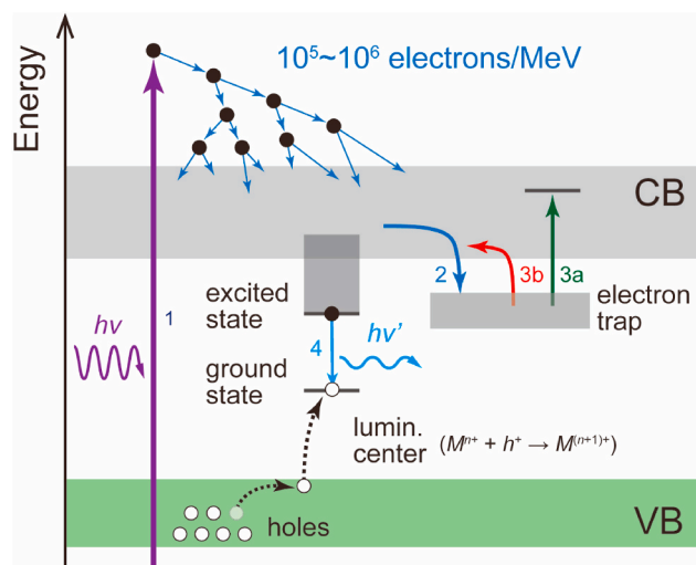
Fig. 1. Schematic illustration of the TL and OSL process, related to the electron trapping and detrapping process: 1. Excitation of electrons with ionizing radiation; 2. Electron trapping; 3a. Optically stimulated electron detrapping; 3b. Thermally stimulated electron detrapping; 4. Radiative electron-hole recombination. During this process, holes generated at the host VB by the ionizing radiation move to the ground state of the luminescence center ion, resulting in the change of the valence state ( M^{n+} + h^+ \rightarrow M^{(n+1)+} ).
