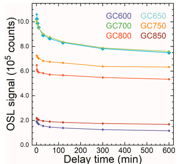
Fig. 8. Fading curves of total OSL signal for all the GC samples.
