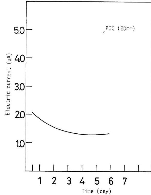
Fig. 6. 35--Typical time dependence of electric current (2)
