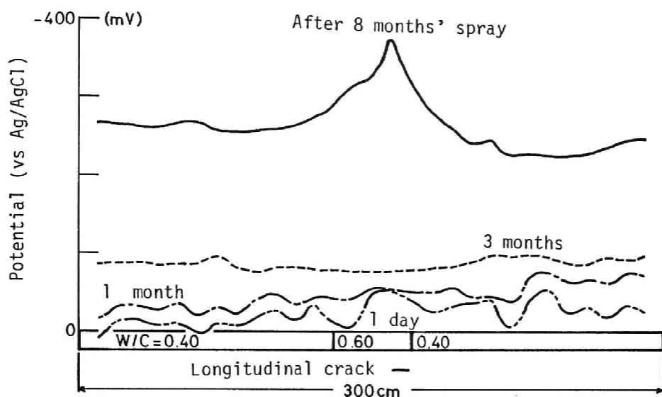
Fig. 7. 6--Potential distribution (Type 0.40-0.60-0.40 specimen)
