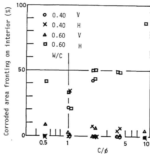
Fig. 6. 15--Influence of C/\phi on corroded area fronting on interior
