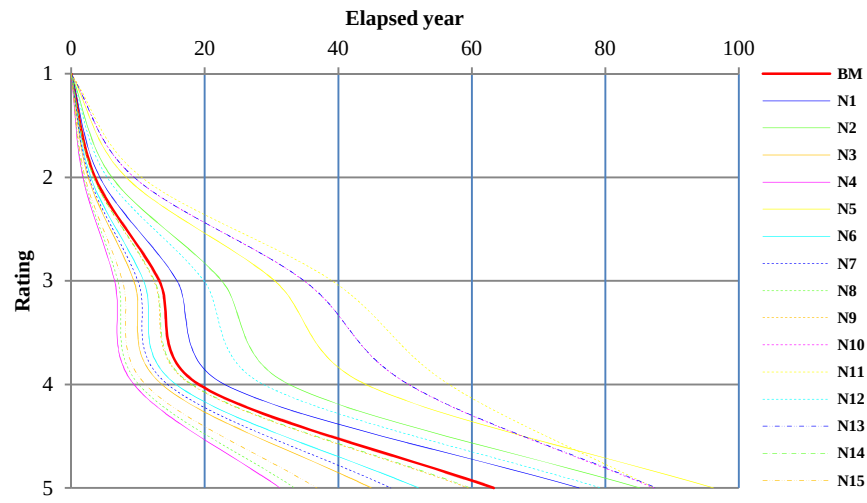
Figure 6.10 Deterioration Curve of Rutting (Practical model case)
