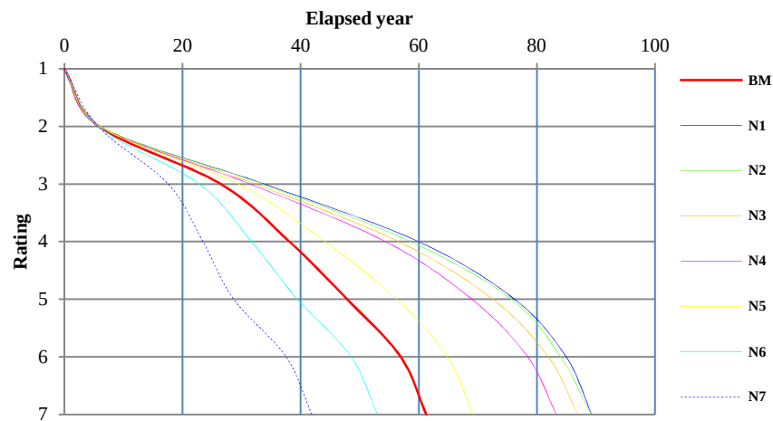
Figure 6.8 Deterioration Curve of Rutting (Kyoto model case)
