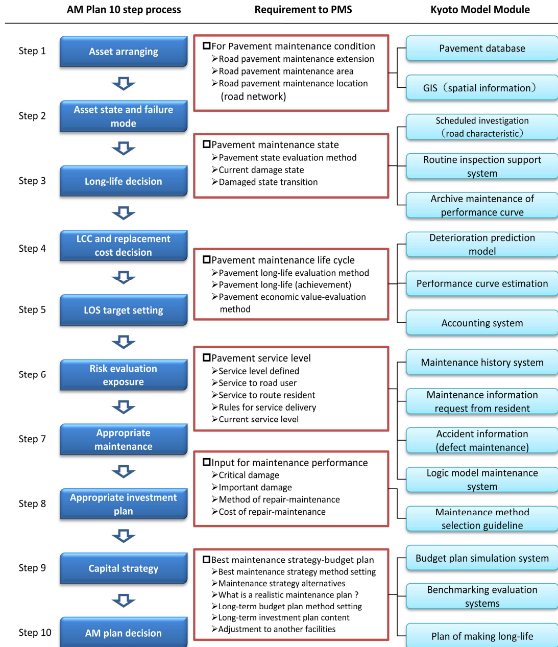
Figure 5.5 Relation among AM Plan Process, Requirement to PMS and Kyoto Model
