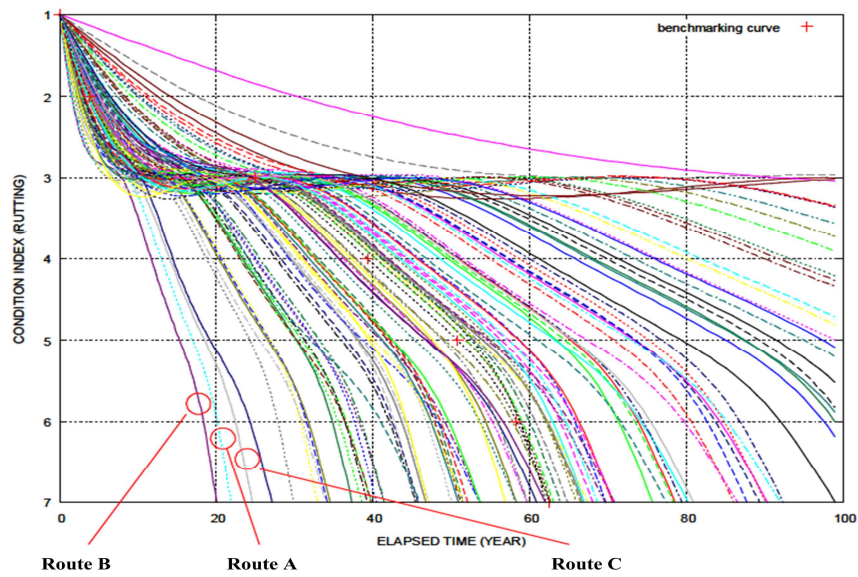
Figure 4.6 Deterioration Curve of Rutting along Route
