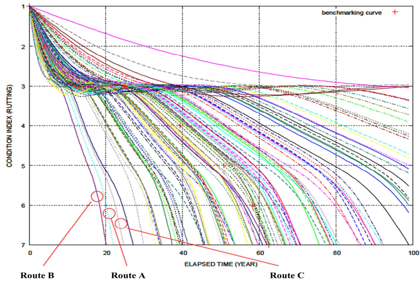
Figure 5.7 Deterioration Curve of Rutting along Route
