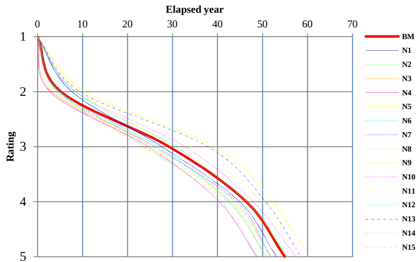
Figure 6.11 Deterioration Curve of Cracking (Practical model case)
