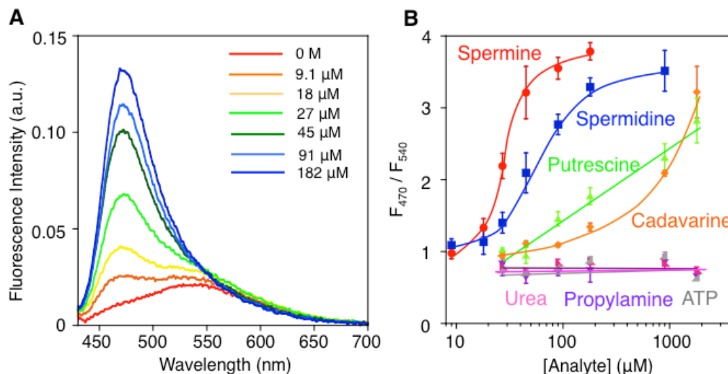
Figure 9. (A) Fluorescence spectral change ( \lambda_{\text{ex}} = 410 nm, MCPD) of G-coum/MTT/hydrogel 1 upon the addition of spermine and (B) fluorescence titration curves (see also Figure S3 for the spectral changes). Lines for spermine and spermidine are best fit of Hill equation to data points. Error bars represent standard deviation ( n = 3 ). Conditions: [1] = 0.18 wt %, [G-coum/MTT] = 0.40 mg/mL, [G-coum] = 0.23 μmol/mg of MMT (19% CEC), 50 mM HEPES (pH 7.4).
