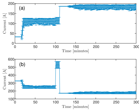
Fig. 4. Ensemble average of the line current with error bars: (a) Line 1 and (b) Line 2.
