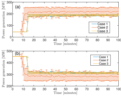
Fig. 2. Ensemble average of the power generation with error bars of (a) Generator 1 and (b) Generator 2.
