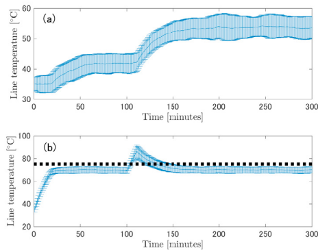
Fig. 5. Ensemble average of the line temperatures with error bars: (a) Line 1 and (b) Line 2. The black dot-line represents the constraint.
