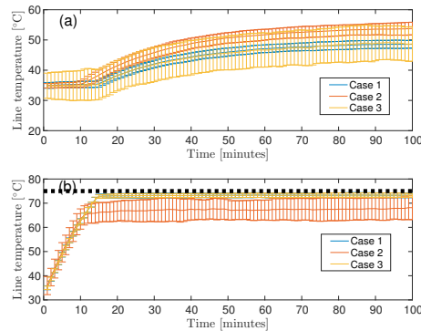
Fig. 3. Ensemble average of the line temperature with error bars of (a) Line 1 and (b) Line 2. The black dot-line represents the constraint.
