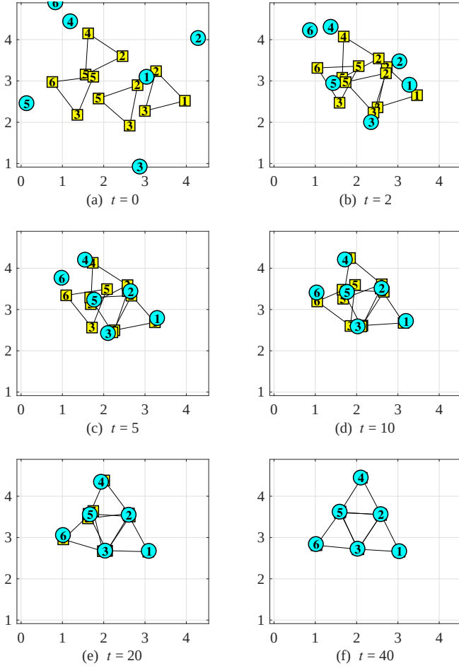
Fig. 8. Snapshots of the simulation: agent positions x_i(t) (circles) and the matched desired positions \hat{x}_{*ik}(t) of each clique C_k (squares).
