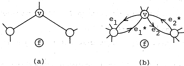
Fig. 4 Common edges of SVE(v) and a face.
