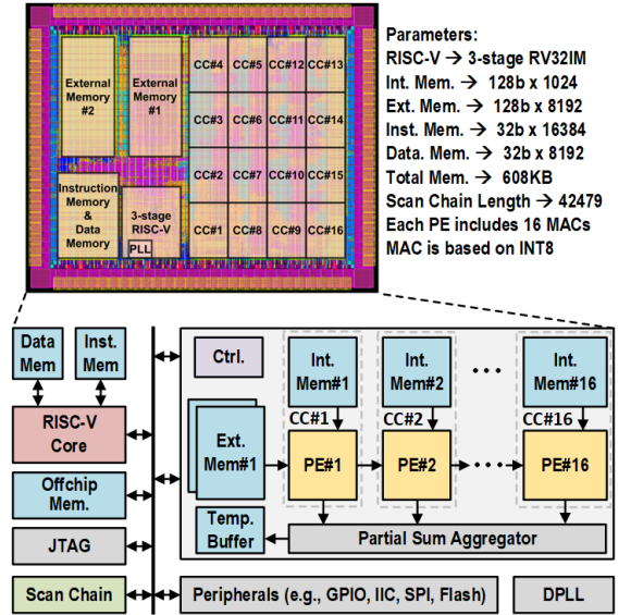
Fig. 2. Edge-AI chip framework.
