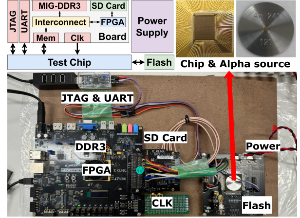
Fig. 3. Experimental setup for alpha irradiation and hardware fault injection.
