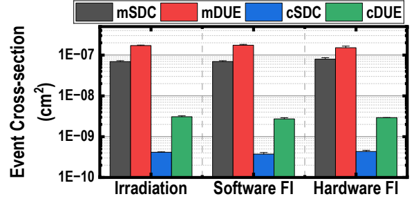
Fig. 4. Cross-section comparison among software FI, hardware FI, and irradiation estimates. The standard deviations for the mSDC, mDUE, cSDC, and cDUE are 5.881e-9, 1.24796e-8, 3.13663e-11, and 1.75107e-10, respectively.
