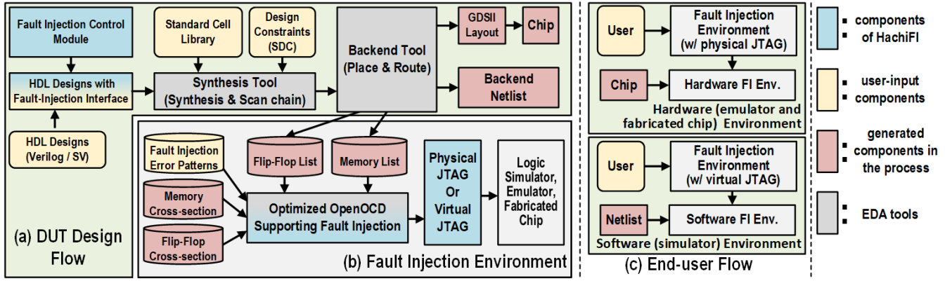
Fig. 1. HachiFI design flow. (a) DUT design flow. (b) Fault injection environment. (c) End-user flow.
