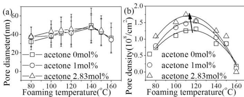
Figure 4.10 Pore size (a) and pore density (b) of nanoporous structure on the cell wall of PC foams
