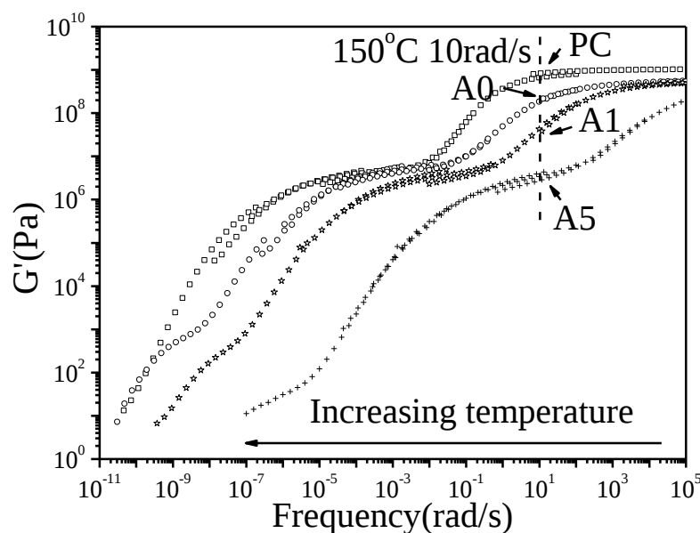
Figure 5.6 Master curves of the G' of PC and PET/PC 30/70 wt% blends (A0, A1 and A5) at 150°C
