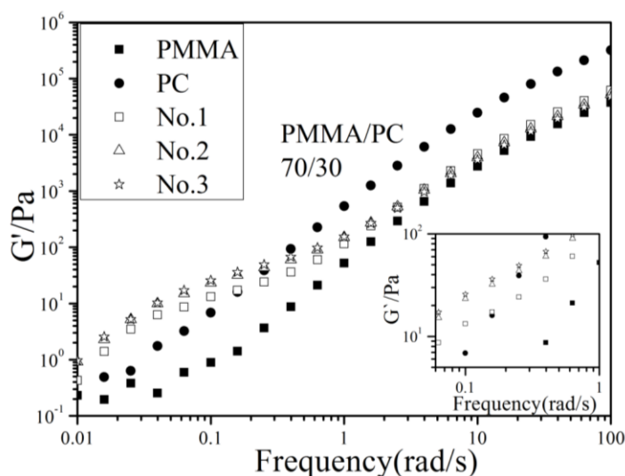
Figure 2.5 Comparison of the dynamic storage modulus curves, G' , of PC, PMMA and 70/30 wt% PMMA/PC blends (No. 1, 2 and 3)
