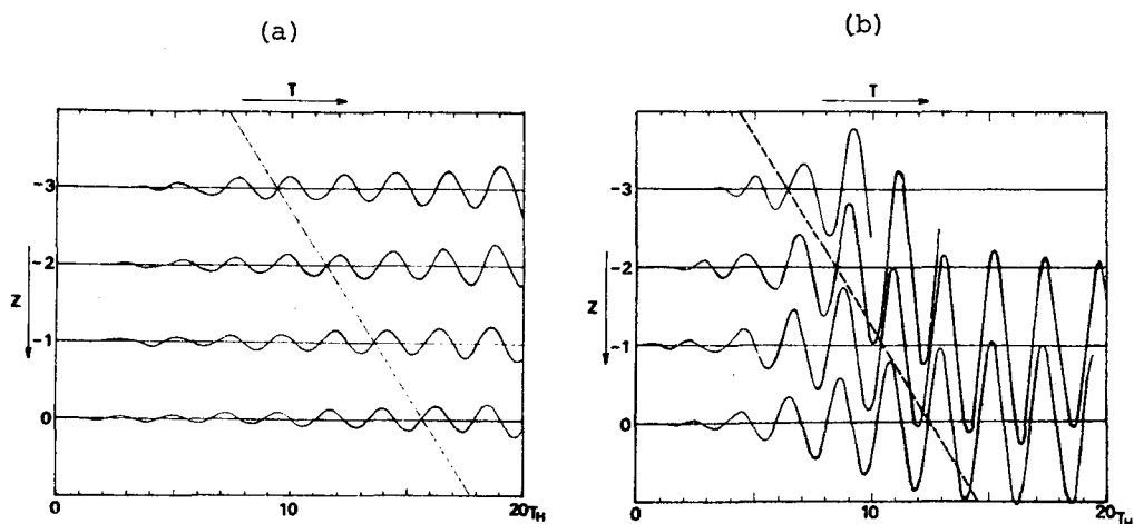
Fig.41 Computed Responses in the Negative z -Space.
