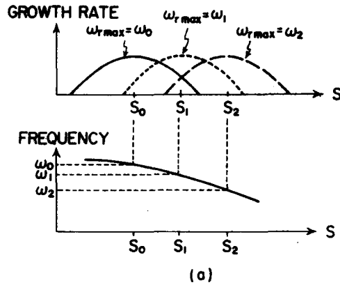
Fig.22 An Illustration of Explaining the Successive Triggering of the Convective Beam Cyclotron Instability in Slowly Varying Inhomogeneous Plasma.
