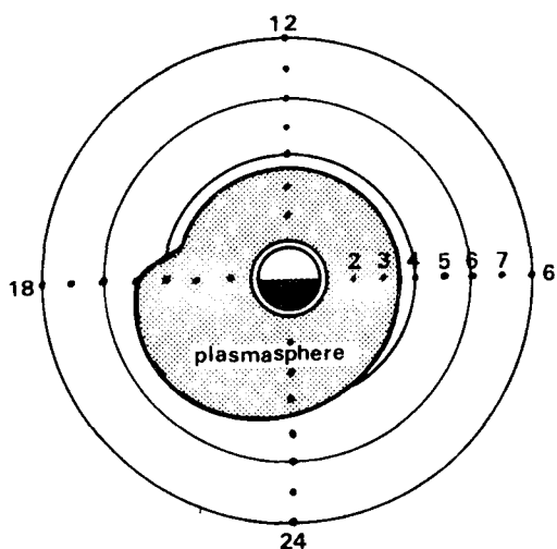
Fig.5 Projection on the Equatorial Plane of the Plasmopause (from Carpenter 12 ).
