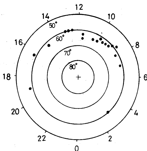
Fig.72 Diurnal Variation of the Background Hiss of Polar Chorus.
