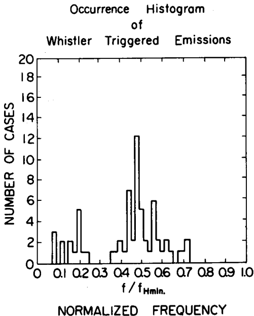
Fig.14 Occurrence Histogram of Whistler Triggered Emissions.
