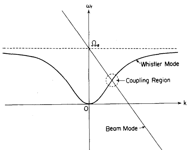
Fig.16 Resonance Condition between the Whistler and the Beam Modes.
