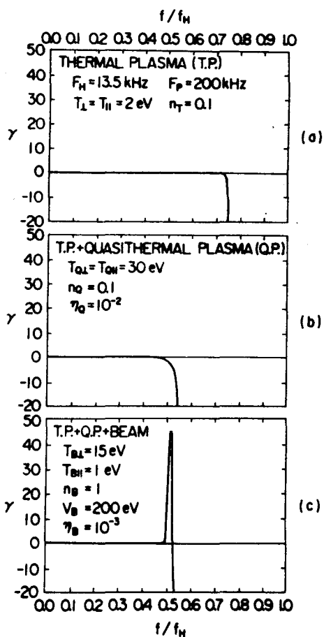
Fig.52 Frequency Characteristics of Whistler Mode Cyclotron Instability for the Model "Triple-Structured" Loss Cone Distribution Function.
