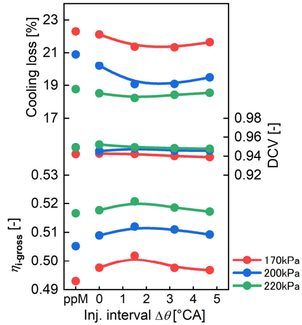
Fig 20. The engine performance against injection interval with various intake pressures.
