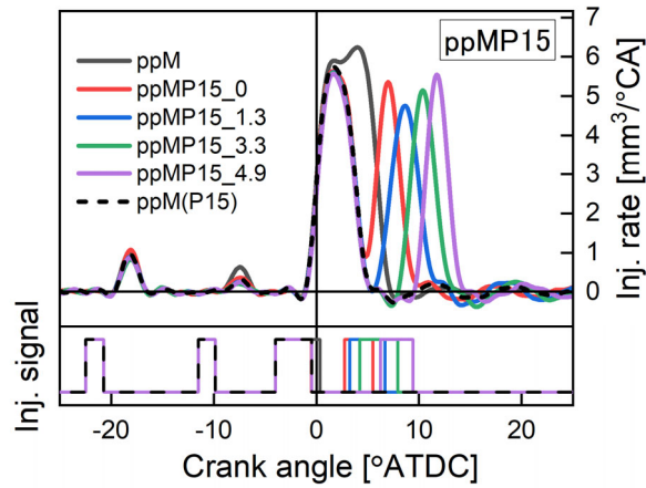
Fig 9. The injection rate with post injection quantity of 15 \text{mm}^3/\text{cycle} .
