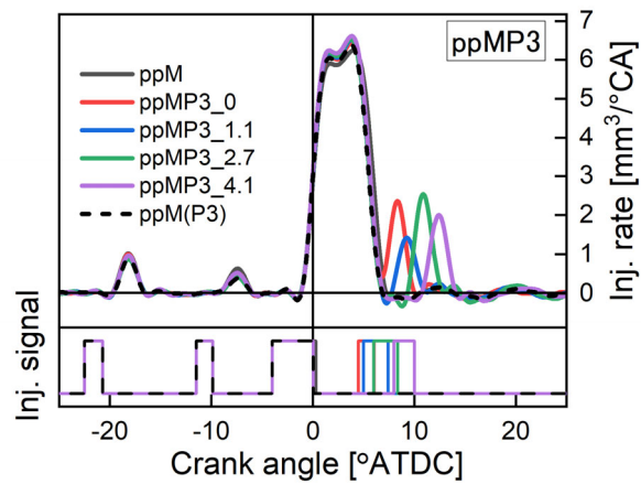
Fig 7. The injection rate with post injection quantity of 3 \text{ mm}^3/\text{cycle} .
