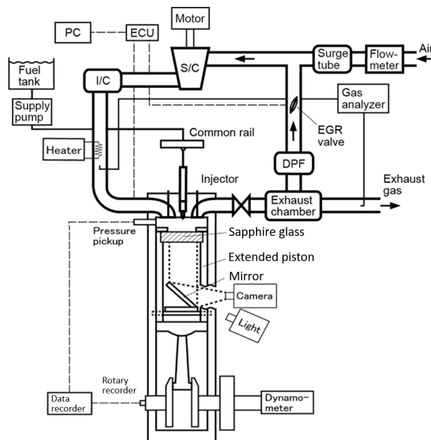
Fig 3. The schematic of experimental setup for the experiments of optical engine.
