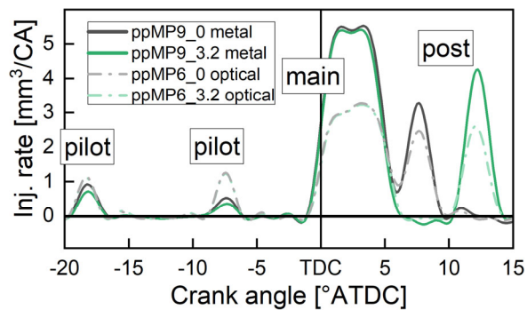
Fig 10. An example of injection rate of metal engine operating condition (solid line) and optical engine operating condition (dashed line).
