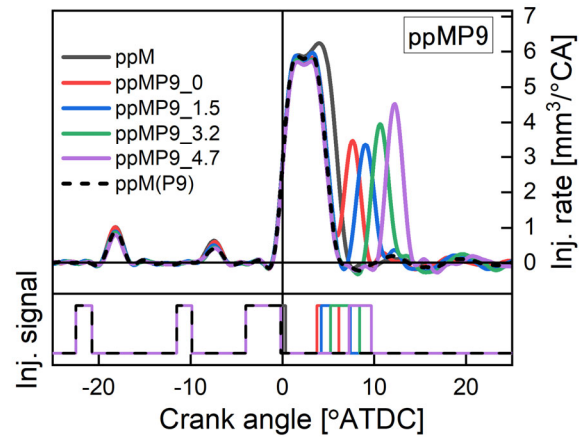
Fig 8. The injection rate with post injection quantity of 9 \text{mm}^3/\text{cycle} .
