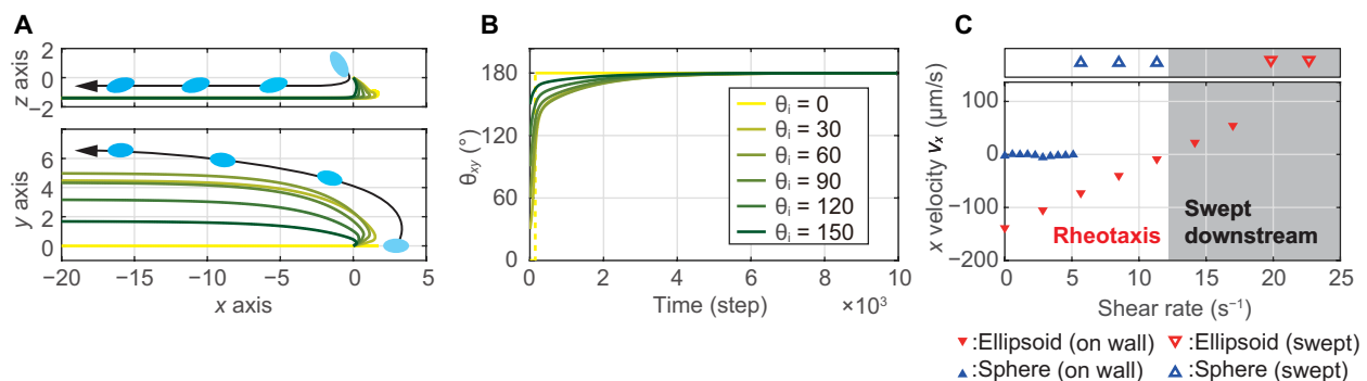
Fig. 5. Evaluation of rheotaxis of numerical swimmers. (A) Dependence of the initial xy angle \theta_i . Top: Trajectories on the xz plane. None of the swimmers detached from the wall. Bottom: Trajectories on the xy plane. In all cases, the swimmers lastly slid against a flow parallel to the x axis. (B) Time evolutions of the xy angle. In all cases, \theta_{xy} converged to 180^\circ . The color depth in the plots denotes the change in \theta_i . In all cases, \dot{\gamma}_* = 0.5 and the initial \theta_{xz} = 60.0^\circ were fixed. (C) The x velocities of the swimmers with the shear rate. The x velocity of the ellipsoidal swimmers with the SBA linearly decreased until \dot{\gamma} = 17.0 \text{ s}^{-1} (filled red triangles). Above \dot{\gamma}_c = 19.8 \text{ s}^{-1} , the ellipsoidal swimmers were swept in the flow; therefore, the velocities were large and positive (empty red triangles). The spherical swimmer stayed on the wall until \dot{\gamma} = 5.1 \text{ s}^{-1} (filled blue triangles) and detached at \dot{\gamma} = 5.7 \text{ s}^{-1} (empty blue triangles). The gray area in the plot represents the shear rate at which the ellipsoidal swimmer was swept downstream including the case with sustaining the slide motion as defined in the experiments.
