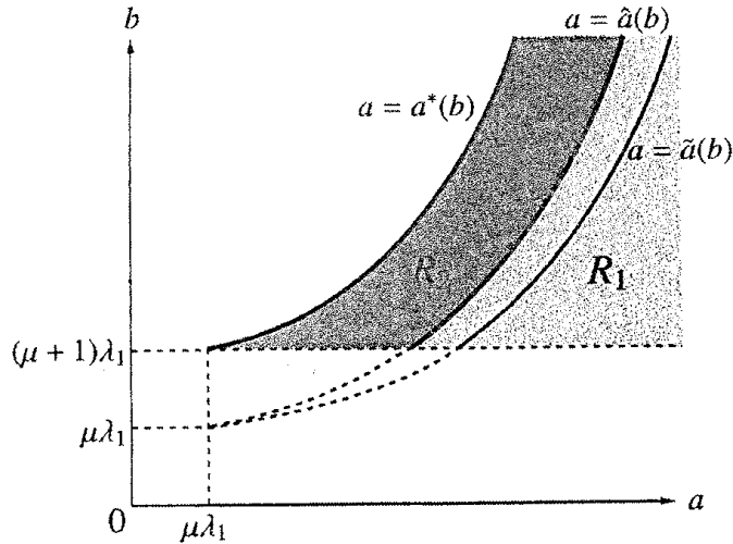
Figure 1: The region R_1 gives the exact coexistence region for (2.2). The region R_2 yields the sufficient condition for existence of positive solutions of (2.3).
