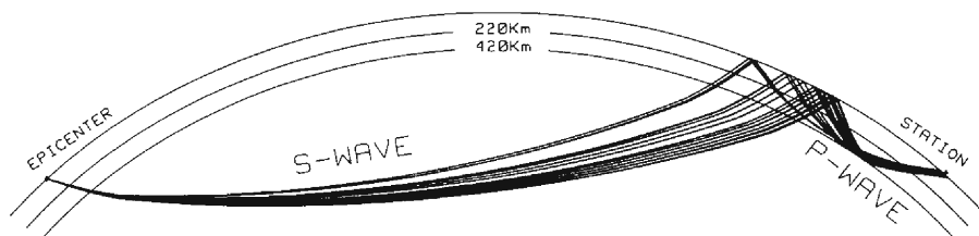
Fig. 11. Seismic rays of SP wave estimated theoretically with PEM-O model based on the ray theory.
