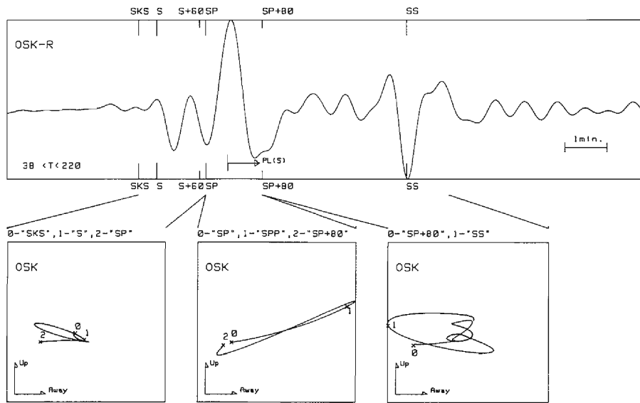
Fig. 10. A longitudinal component of X_1 recorded at OSK, particle orbits in the vertical plane parallel to the direction of the epicenter. Theoretically estimated arrival times of mS_nP are exhibited on the seismogram and particle orbits.
