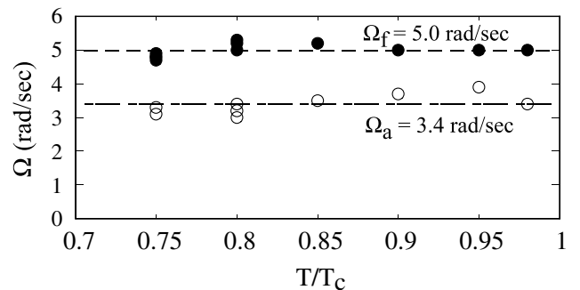
FIG. 4. The critical speed for vortex formation \Omega_f shown by solid circles and annihilation \Omega_a shown by open circles as a function of temperature for type A texture.
