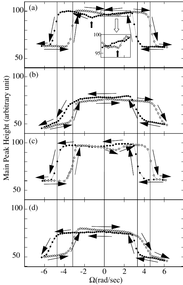
FIG. 3. NMR absorption of the main peak at R_t^2 = 1.0 as a function of rotation speed \Omega during acceleration and deceleration cycle. The conditions of cooling the sample through T_c are: (a) (+2 rad/sec, -22 mT), (b) (+2 rad/sec, +22 mT), (c) (-2 rad/sec, +22 mT), (d) (-2 rad/sec, -22 mT). The spectra (a) and (c) correspond to type A texture and (b) and (d) to type B. Thin arrows indicate the direction of taking data and vertical lines are \Omega_f and \Omega_a for type A.
