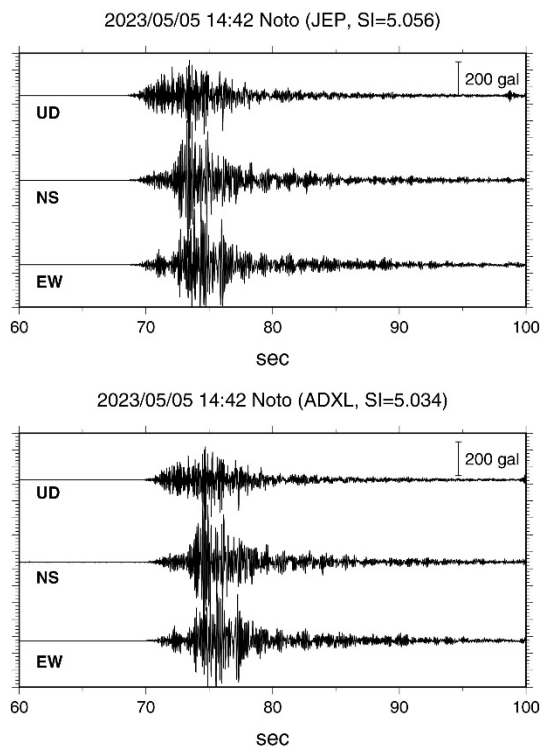
Fig.5 : Waveform of the M6.5 earthquake at 14:42 on 2023/05/05 observed at DP.HRJ. The upper waveform is observed by JEP-8E3 and the lower one by ADXL355.
