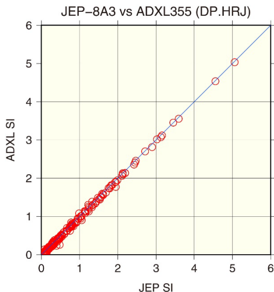
Fig.6 : Comparison of calculated seismic intensity by simultaneous observation of JEP-8A3 and ADXL355 at DP.HRJ.
