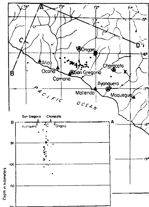
Fig. 8 The San Agustin fault zone revealed by the locations of epicenters (dots) which determined from the four seismograph stations in Arequipa Region ×, ▲ : epicenter of destructive earthquake, seismograph station Lower : vertical cross section (AB) across the fault zone showing distribution of hypocenters
