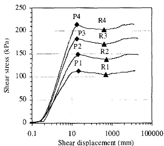
Fig. 4 Results of drained monotonic ring shear tests for normally consolidated silica sand no. 6 under effective stress levels of 147 kPa ( e_c=0.97 ), 196 kPa ( e_c=0.98 ), 245 kPa ( e_c=0.96 ) and 294 kPa ( e_c=0.94 ).
