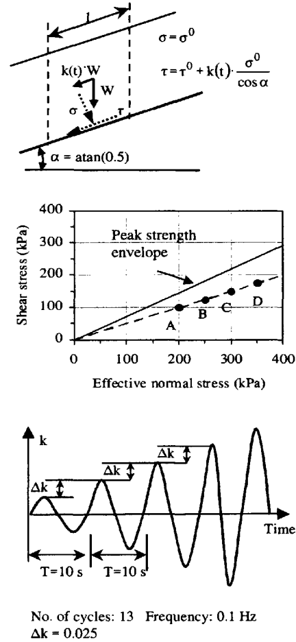
Fig. 7 Initial stress conditions (a), (b) and wave form of cyclic shear stress (c) for undrained cyclic loading ring shear tests
