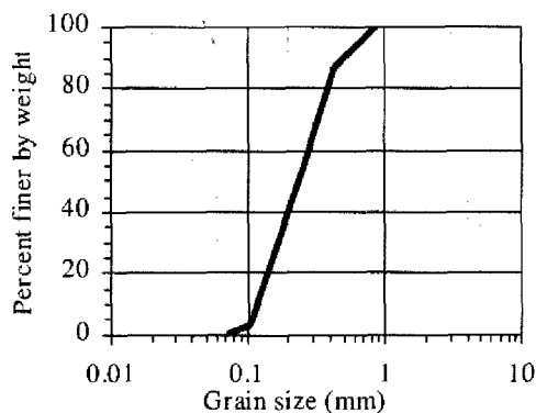
Fig. 3 Grain-size distribution of silica sand no. 6
