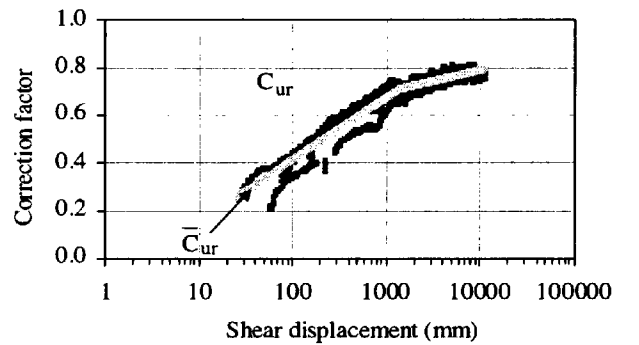
Fig. 14 Correction factor in relation with shear displacement
