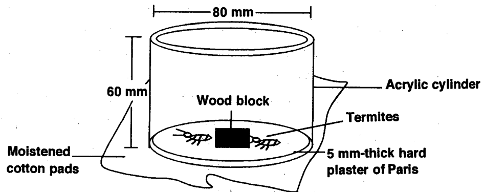
Fig. 1. An acrylic test container for wood block test (JWPA-test).
