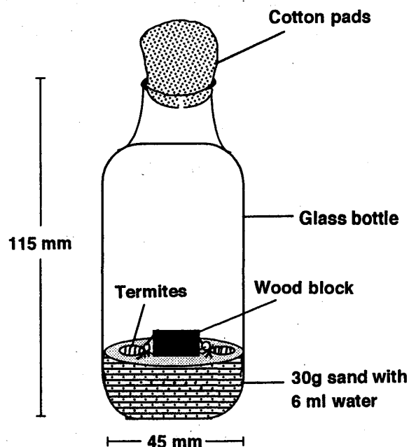
Fig. 2. An glass bottle container for modified wood block test (MWBT).
