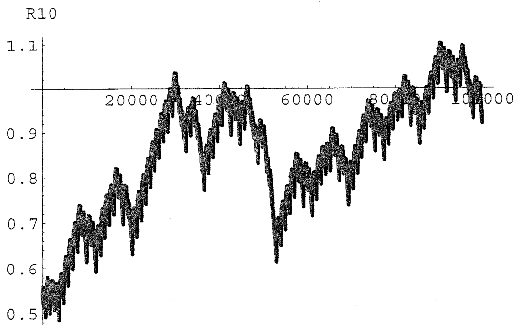
Figure 15: Mori , ratio: the first 100000
