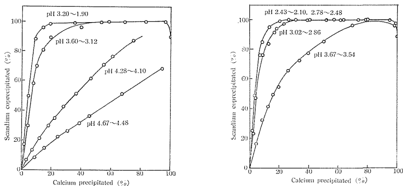
Fig. 1. Coprecipitation of scandium with calcium oxalate at different pH.
