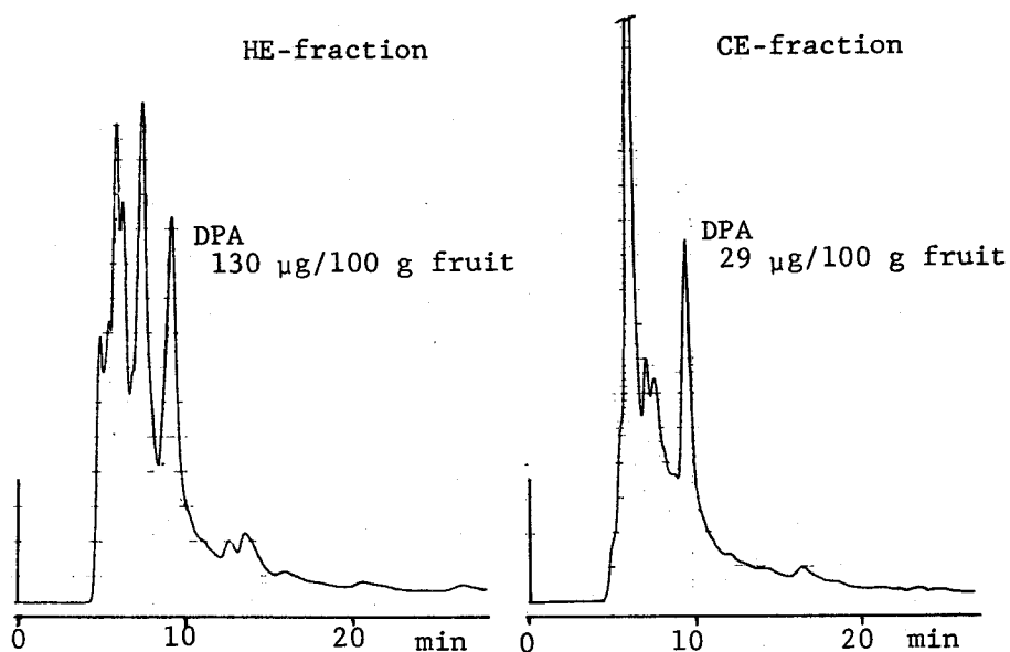
Figure IV-3 HPLC trace of HE- and CE-fraction of avocado fruit. HPLC condition, see Figure IV-1; injection volume, HE-fraction: 1 \mu\text{l} , CE-fraction: 3 \mu\text{l} .
