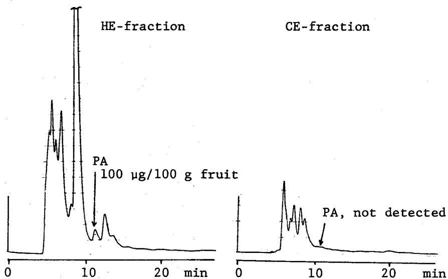
Figure IV-4 HPLC trace of HE- and CE-fraction of cherry fruit. HPLC condition, see Figure IV-1; injection volume, HE-fraction: 2 \mu\text{l} , CE-fraction: 2 \mu\text{l} .
