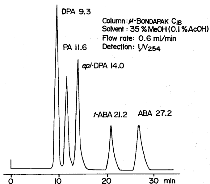
Figure IV-1 HPLC separation of ABA metabolites.
