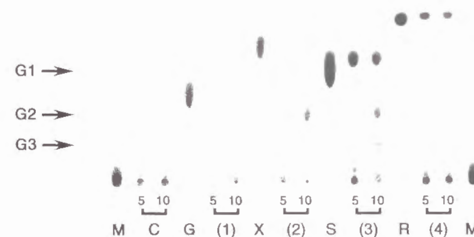
Fig. 7. TLC Patterns of Transglycosylation to Various Saccharides.
