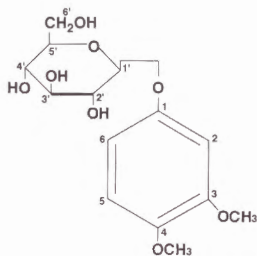
Fig. 4. Structure of 3,4-Dimethoxyphenyl- O - \beta -D-glucopyranoside.
