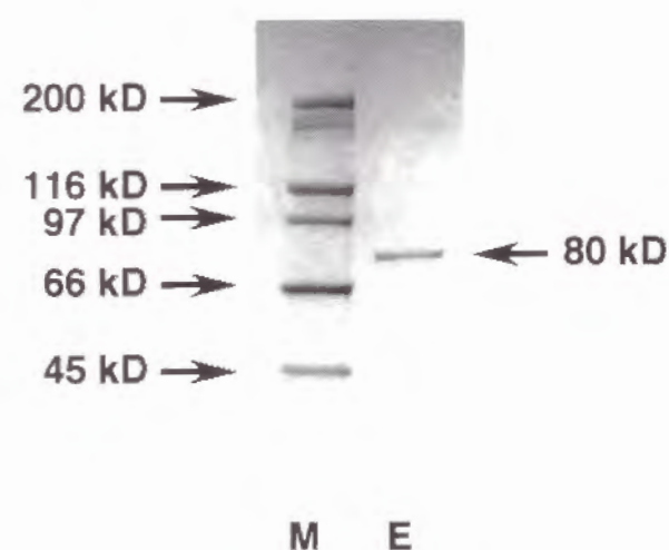
Fig. 1. SDS-PAGE of Purified CGTase from an Alkalophilic Bacillus sp. E, purified CGTase; M, marker proteins; myosin ( Mr , 200,000), E. coli \beta -galactosidase ( Mr , 116,250), rabbit muscle phosphorylase b ( Mr , 97,400), bovine serum albumin ( Mr , 66,200), and hen egg white ovalbumin ( Mr , 45,000).
