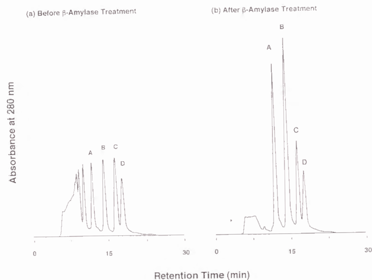
Fig. 4. HPLC(ODS) Patterns of Hesperidin Glycosides before and after \beta -Amylase Treatments.
