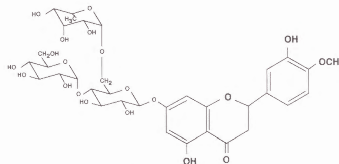
Fig. 5. Structure of glycoside C.
