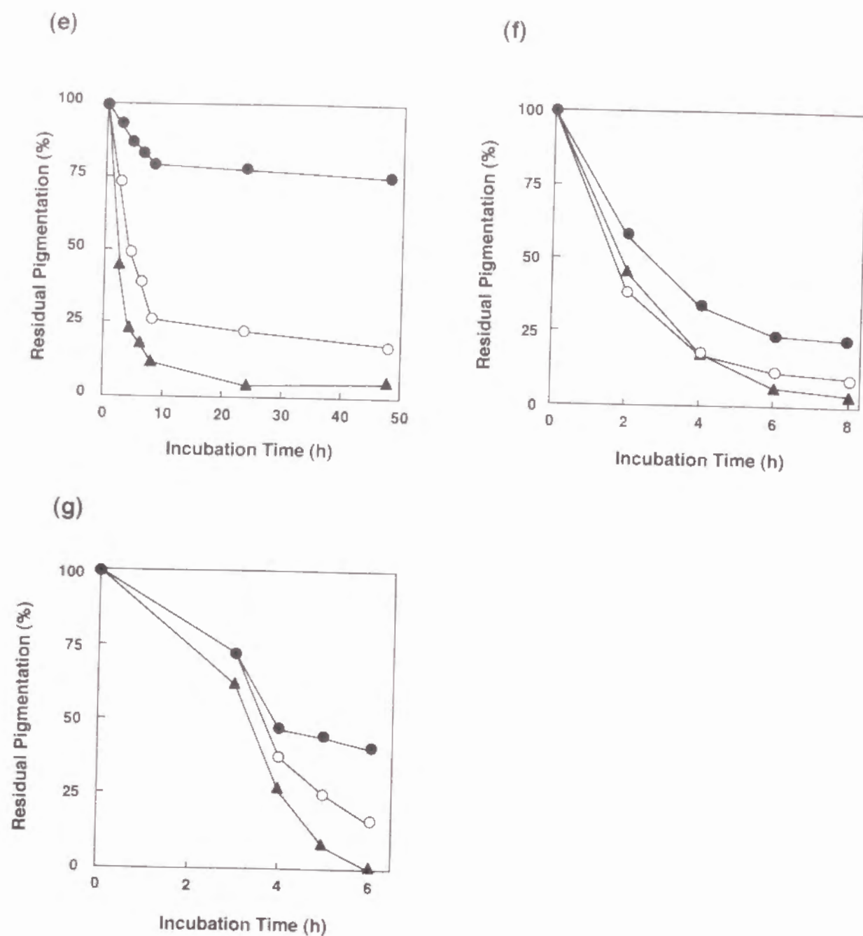
Fig. 8. Stabilization of the Pigmentation of Various Pigments by Hesperidin Glycosides.
