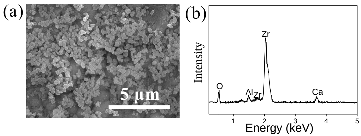
Figure 3 (a) SEM image and (b) EDX profile of the doubled sandblasted zirconia specimens after AN treatment.
