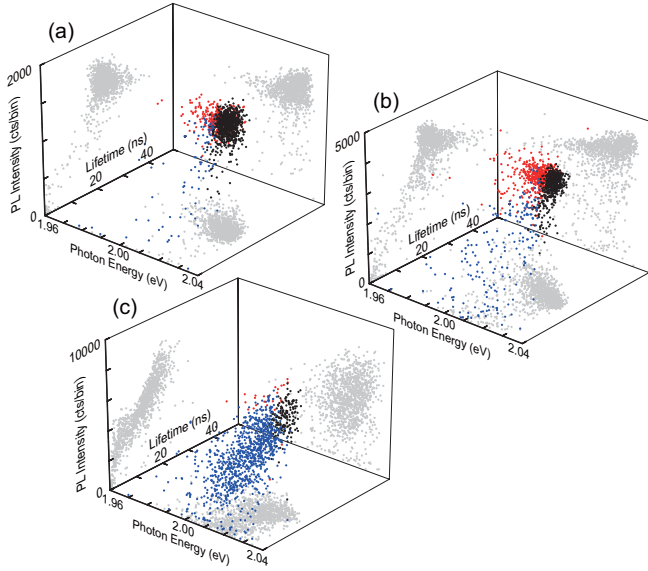
FIG. 4. (Color online) Three-dimensional plots to represent the relationships between photon energy, lifetime, and intensity measured under the elevated excitation power at (a) 0.8, (b) 2.6, and (c) 6.6 \mu\text{W} .
