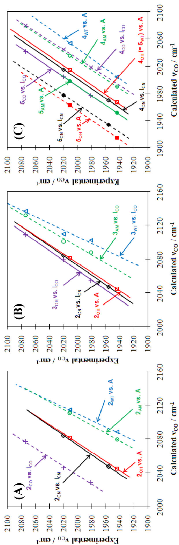
Figure 2. Calculated CO stretching frequencies v_{CO} of various model compounds vs. experimental data, 7 (A) 2x vs. A, (B) 3x vs. I_{CO} , and (C) 4x (or 5x) vs. A. Solid and dashed lines indicate successful relation and unsuccessful one, respectively.
