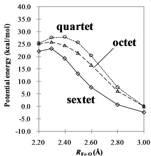
(B) On the sextet geometry
