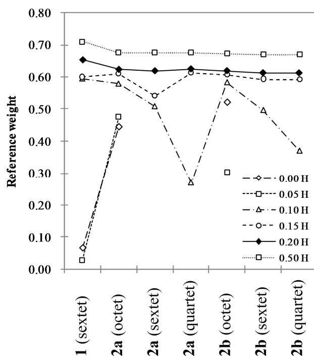
Figure A4. Reference weights calculated by the LS-CASPT2 method with several level shifts. In no shift and very small shift value of 0.05 E_h , some of data could not be presented because the CASPT2 iteration was not converged, indicating that there are strong intruder states and the reference weights are too small in some calculations. Note that the reference weights are not constant where the shift value is less than 0.20 E_h , because the intruder states are not completely reduced with such shift value.
