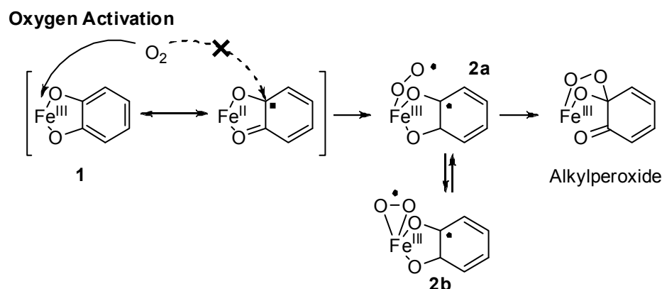
Scheme 10. Proposed mechanism of the dioxygen activation in iron(III) catechol dioxygenase
