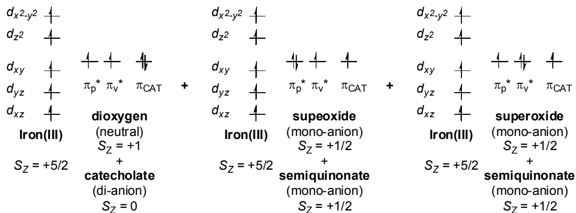
(A) octet spin state ( S_Z = +7/2 )
