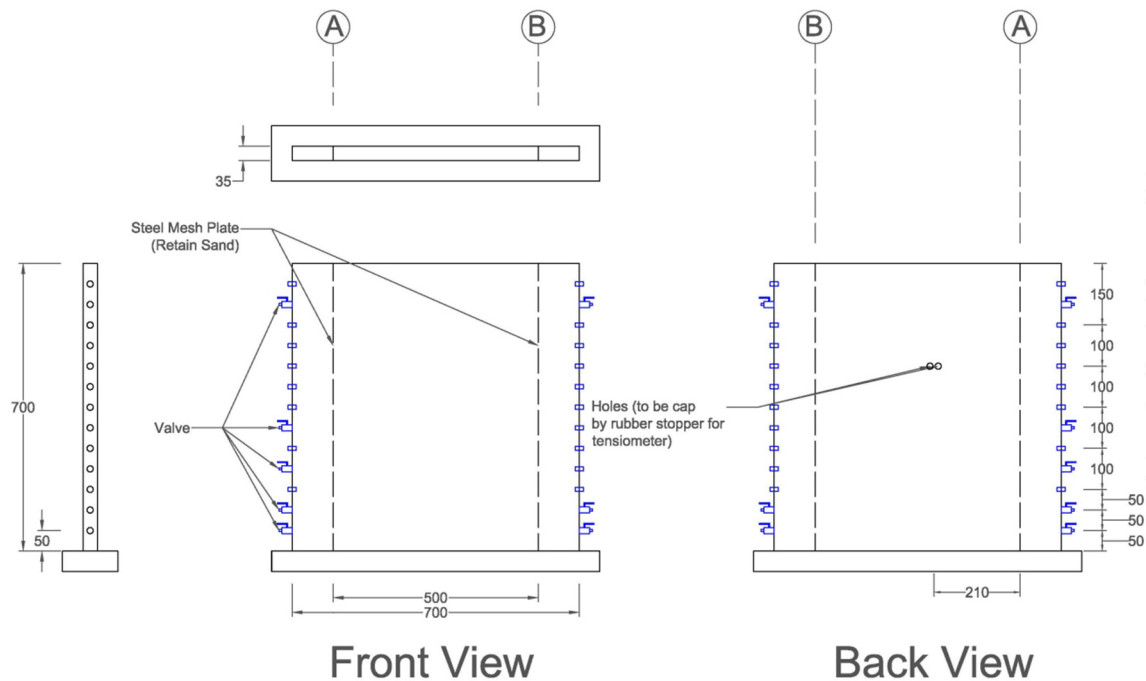
Figure 5.1 Tank design.
