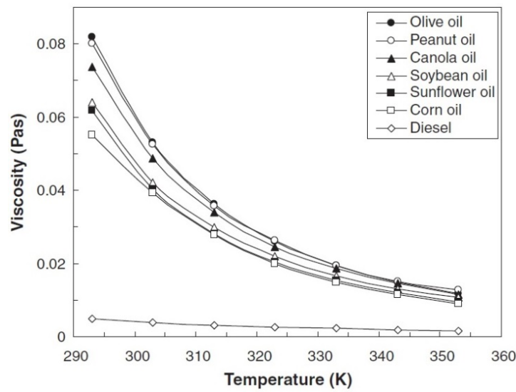
Figure 2.2 Variation of various oil viscosities in temperature (Franco and Nguyen 2011).
