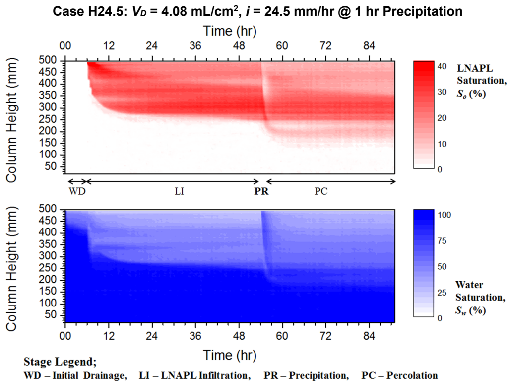
Figure 4.7 LNAPL and water saturation profile for case H24.5.
