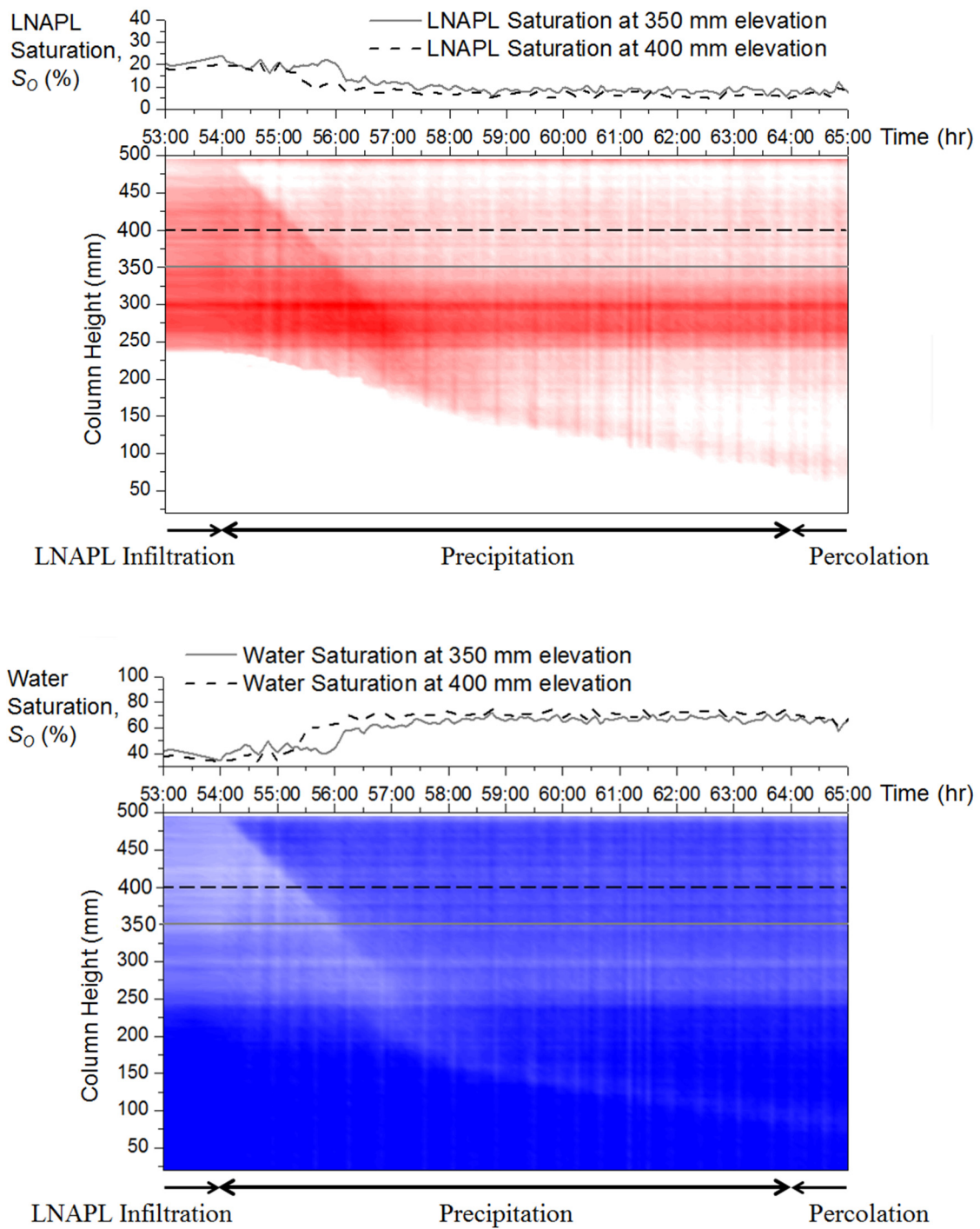
Figure 4.16 Saturation profile of one hour before and after precipitation, as well as during precipitation (10 hours) for the case H6.5V: (a) LNAPL saturation profile and (b) water saturation profile.
