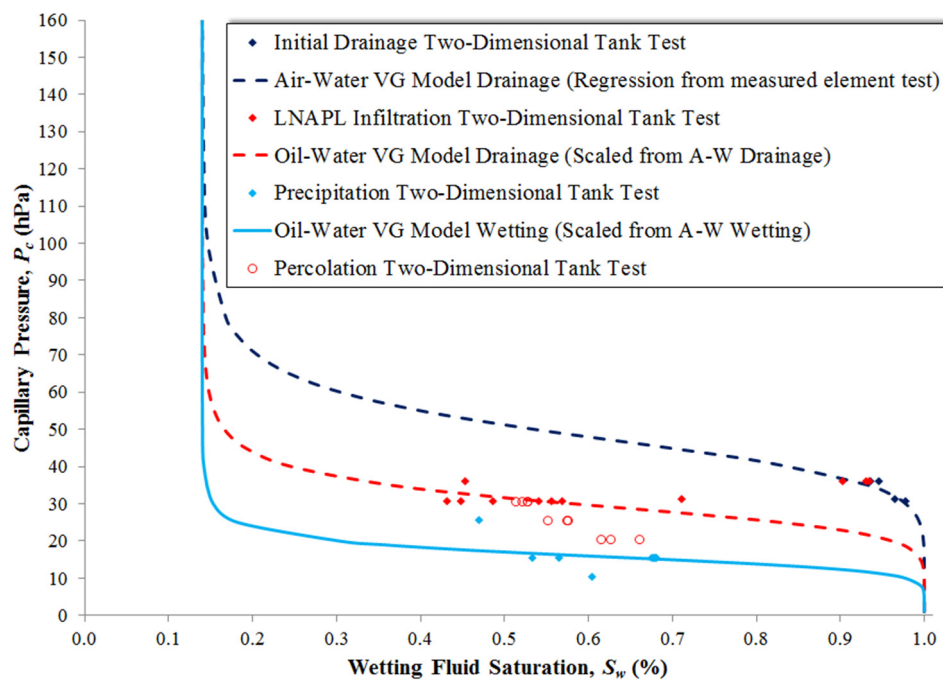
Figure 5.14 S - p relations for tank test during percolation stage.
