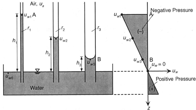
Figure 2.7 Analogy of capillary pressure at various sizes of the capillary tube (Lu and Likos 2004).
