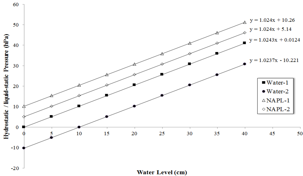
Figure 3.3 Calibration results.
