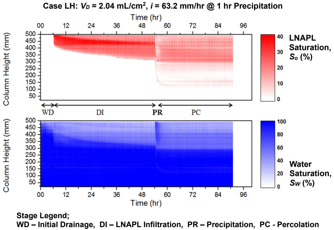
Figure 3.15 LNAPL and water saturation profile for case LH.
