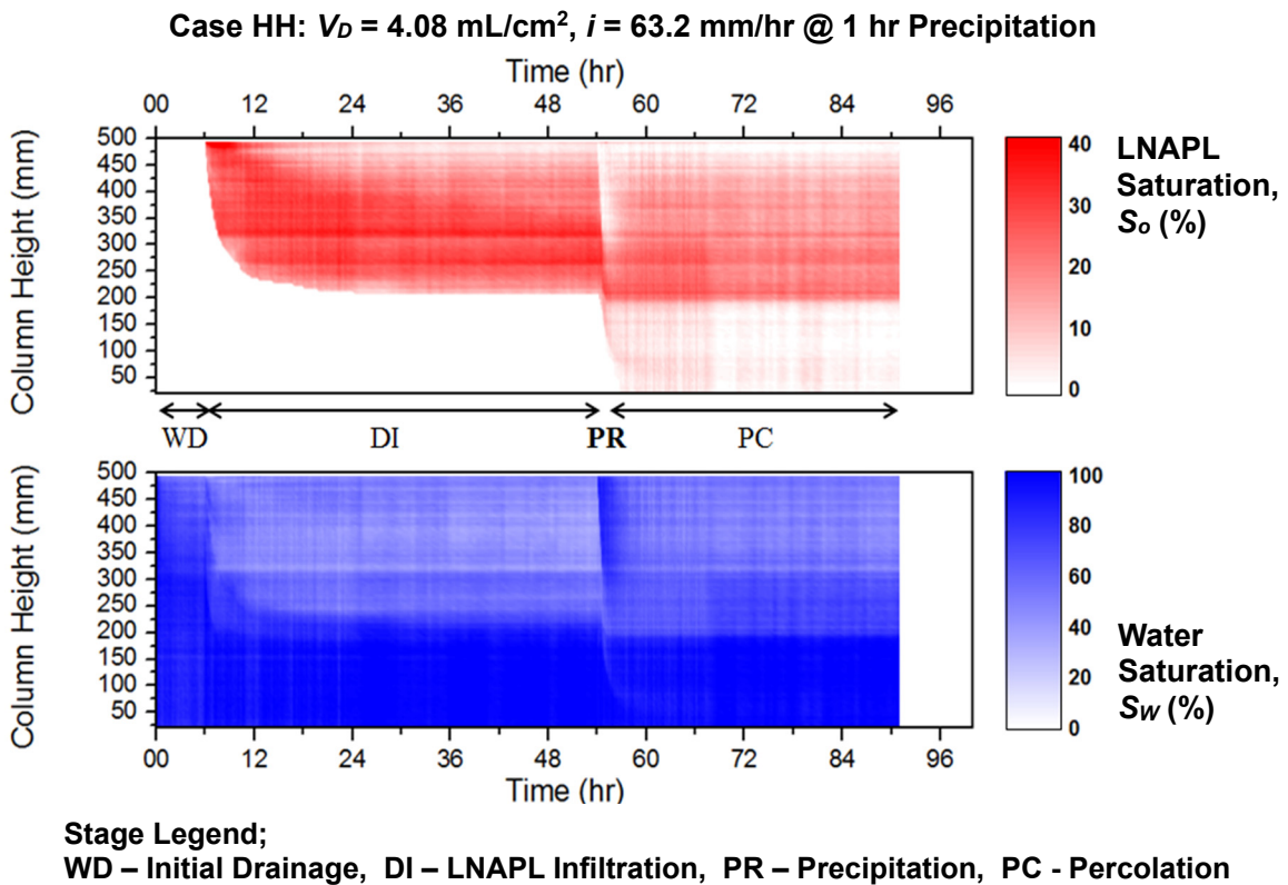
Figure 3.16 LNAPL and water saturation profile for case HH.
