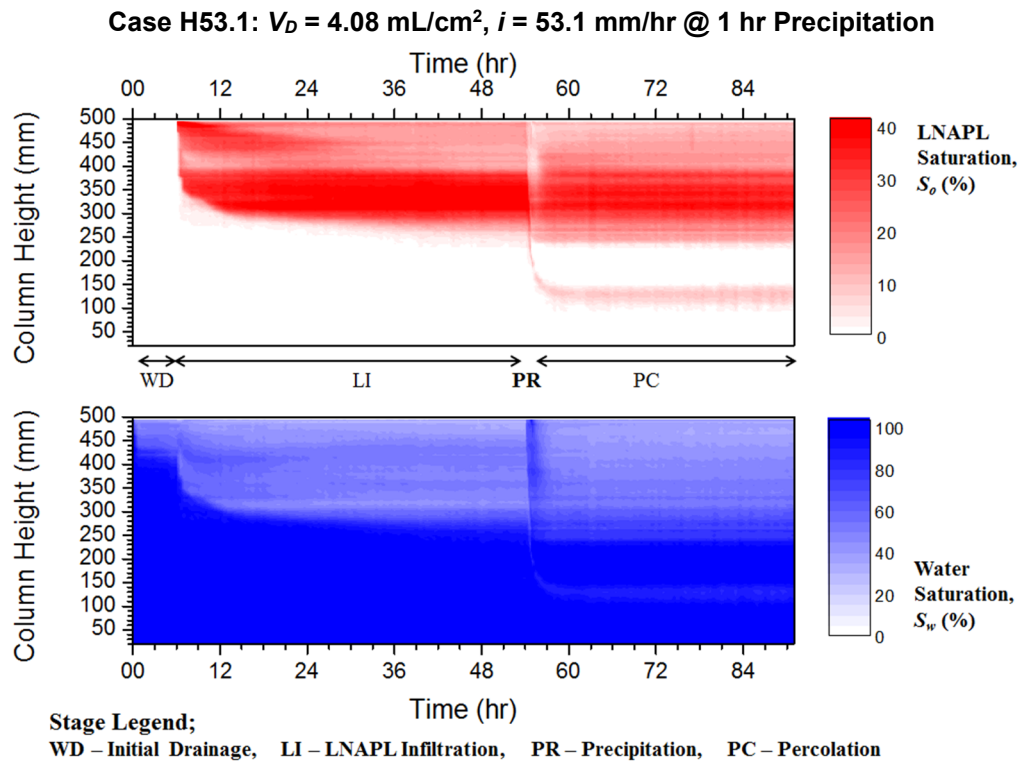
Figure 4.6 LNAPL and water saturation profile for case H53.1.
