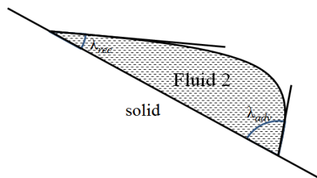
Figure 2.6 Nonuniqueness of contact angle for a moving liquid phase.
