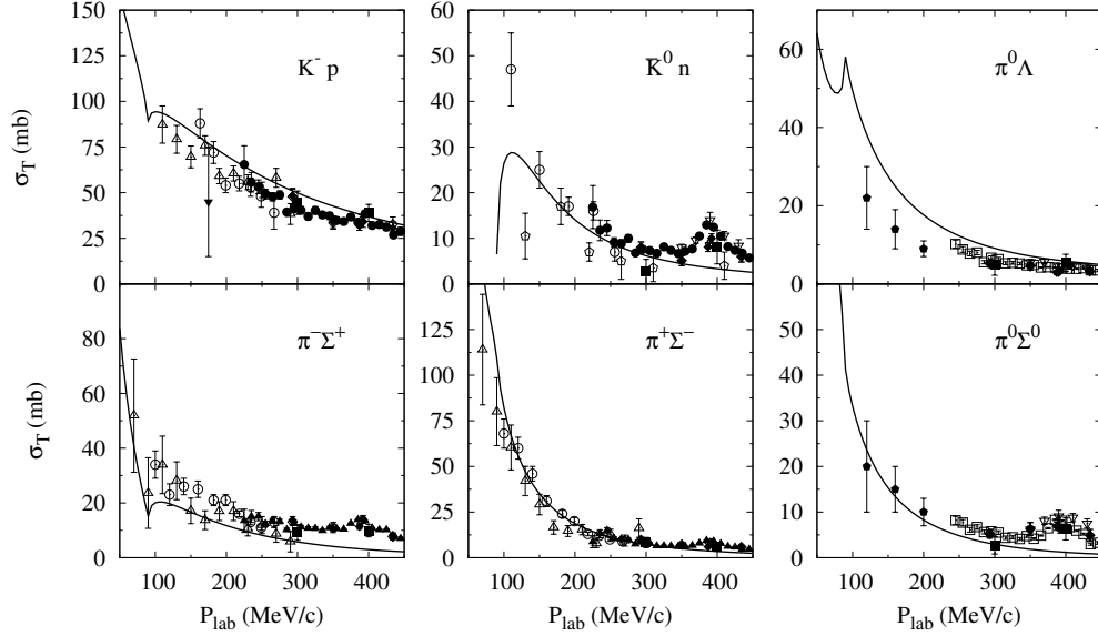
Figure 5: Total cross sections of K^-p to K^-p , \bar{K}^0n , \pi^0\Lambda , \pi^-\Sigma^+ , \pi^+\Sigma^- and \pi^0\Sigma^0 . The solid lines denote the results of the chiral unitary model [137, 143]. The symbols stand for data points taken from Refs. [38, 44, 43, 42, 144, 145, 146, 147, 148, 149, 40].
