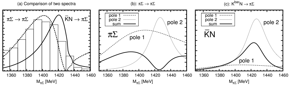
Figure 7: \pi\Sigma invariant mass spectra with I = 0 in arbitrary units taken from Ref. [150]. See also Ref. [11]. (a): chiral unitary model calculation of the \pi\Sigma invariant mass spectra of \bar{K}N \rightarrow \pi\Sigma (solid line) and \pi\Sigma \rightarrow \pi\Sigma (dashed line). The heights are adjusted. The histogram denotes an experimental spectrum of \pi^-\Sigma^+ channel given in Ref. [25]. (b) and (c): model calculations of the \pi\Sigma spectra by two Breit-Wigner terms whose parameters are determined by the chiral unitary model. The dashed (dotted) line denotes the spectrum only with pole 1 (pole 2) term, while the solid line shows the spectrum calculated by coherent sum of pole 1 and 2.
