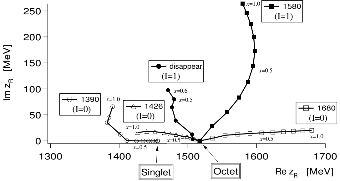
Figure 8: Trajectories of the poles in the scattering amplitudes obtained by changing the SU(3) breaking parameter x gradually. In the SU(3) symmetric limit ( x = 0 ), only two poles appear, one is for the singlet and the other for the octet. The symbols correspond to the step size \delta x = 0.1 . Figure is taken from Ref. [11].
