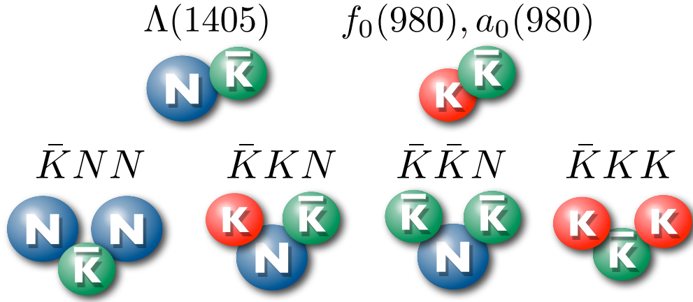
Figure 15: Family of kaonic few-body states.
