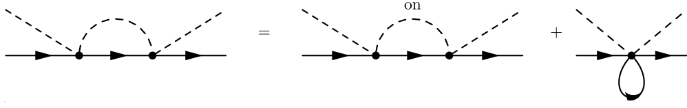
Figure 4: Diagrammatic illustration of the on-shell factorization of Eq. (23).
