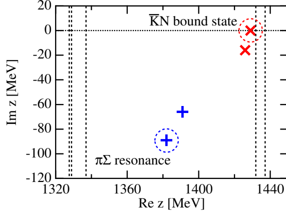
Figure 9: Pole positions of the scattering amplitude for \Lambda(1405) in the complex energy plane with the parameters in Ref. [137]. Crosses enclosed by circles represent poles obtained by switching off the transition couplings. Vertical dashed lines indicate the meson-baryon threshold energies.
