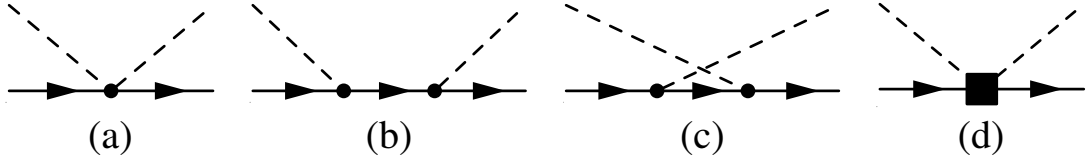
Figure 1: Feynman diagrams for the meson-baryon interactions in chiral perturbation theory. (a) Weinberg-Tomozawa interaction, (b) s-channel Born term, (c) u-channel Born term, (d) NLO interaction. The dots represent the \mathcal{O}(p) vertices while the square denotes the \mathcal{O}(p^2) vertex.
