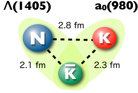
Figure 16: Schematic structure of the \bar{K}KN quasi-bound state with the inter-hadron distances.
