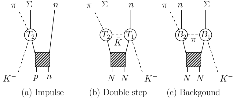
Figure 10: Feynman diagrams for the K^-d \rightarrow \pi\Sigma n reaction to observe the \Lambda(1405) resonance in the \pi\Sigma invariant mass spectrum [160]. The diagrams (a) and (b) correspond to the impulse approximation and the double step process, respectively, in which T_2 is the scattering amplitude for \bar{K}N \rightarrow \pi\Sigma involving the \Lambda(1405) resonance and T_1 is for \bar{K}N \rightarrow \bar{K}N . The diagram (c) is a possible background contribution with one \pi exchange, in which the final \pi\Sigma does not come from \Lambda(1405) .
