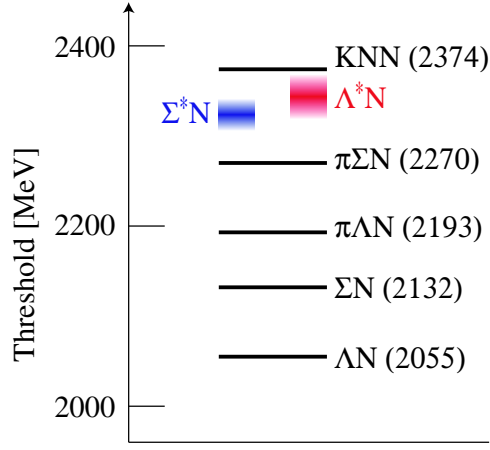
Figure 14: Threshold energies of multihadron channels below the \bar{K}NN threshold. \Lambda^* and \Sigma^* represent \Lambda(1405) ( J^P = 1/2^- ) and \Sigma(1385) ( J^P = 3/2^+ ), respectively.
