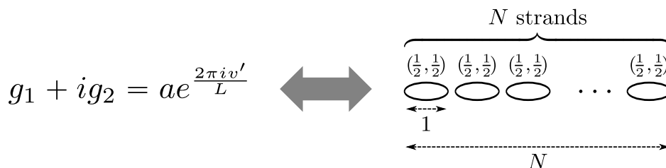
Figure 2. The state/geometry dictionary for the maximally-spinning supertube with dipole charge 1. The circular profile given in (3.1) on the gravity side (shown on the left) corresponds to the CFT state with N strands all with length one and R-charge eigenvalues (j_\ell, \tilde{j}_\ell) = (\frac{1}{2}, \frac{1}{2}) (shown on the right).
