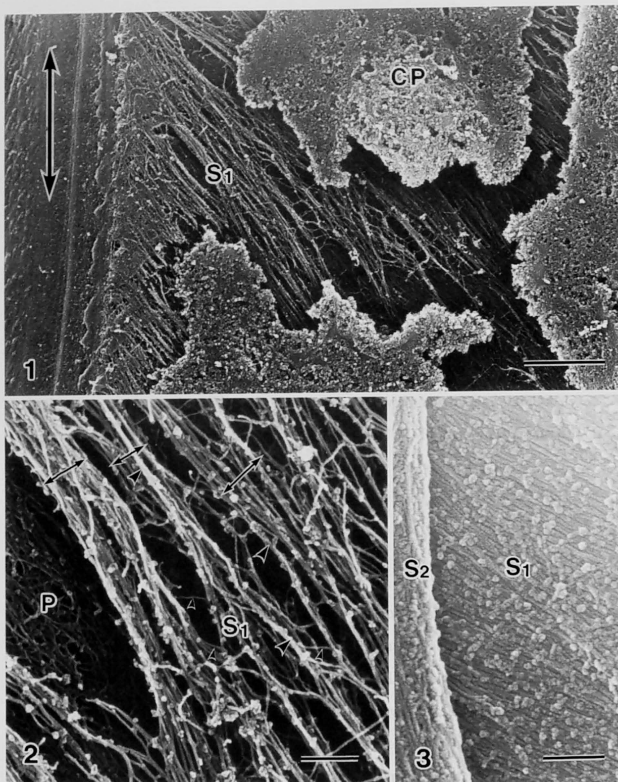
Fig. 3.1 Overview of S_1 -forming fiber. Cytoplasm was often found on the inner surface of the secondary cell wall. An arrow indicates direction of fiber axis. Bar = 2 \mu m.
