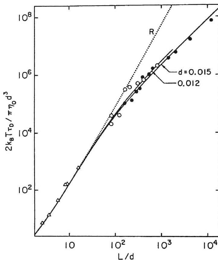
Fig. 4.12. Double logarithmic plots of 2k_B T \tau_D / \pi \eta_0 d^3 against L/d for stiff chains ( \kappa_0=0 and \alpha=\Delta=0^\circ ). The open and filled circles and triangles represent the experimental values of Sakamoto et al. (Ref. 42) for DNA in 1 mM NaCl at 10^\circ\text{C} , of Bur and Roberts (Ref. 43) for poly( n -butyl isocyanate) in carbon tetrachloride at 22.9^\circ\text{C} , and of Matsumoto et al. (Ref. 44) for poly( \gamma -benzyl L -glutamate) in m -cresol at 25^\circ\text{C} , respectively. The full curves represent the best fit theoretical values calculated from Eq. (4.39), and the dotted curve R the values from Eq. (4.40) for the spherocylinder.
