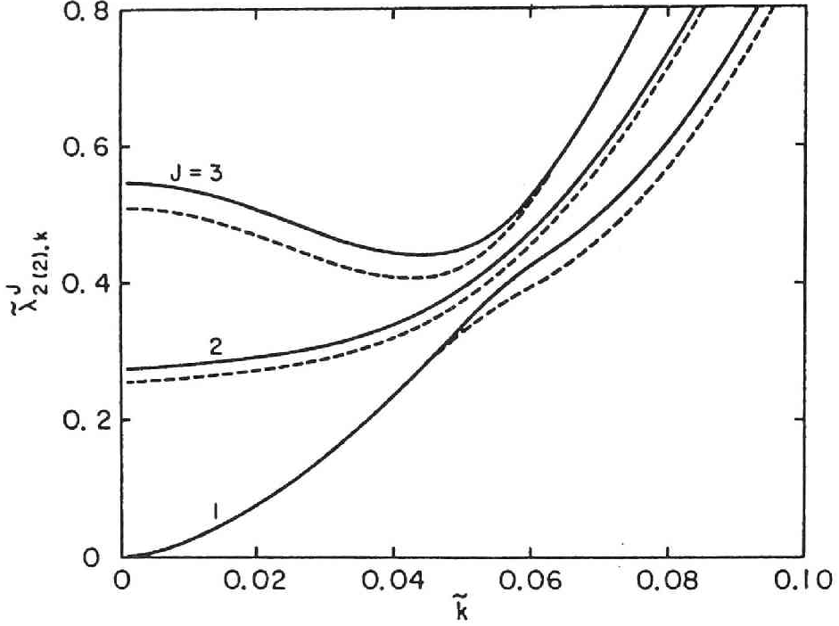
Fig. 5.1. The reduced eigenvalues \tilde{\lambda}_{2(2),k}^{(J)} ( J=1, 2, 3 ) plotted against the reduced wave number \tilde{k} for syndiotactic polystyrene with n_b=2 , N=999 , r_1=1 , and r_2=15 . The full and broken curves represent the values calculated following procedures B and A, respectively.
