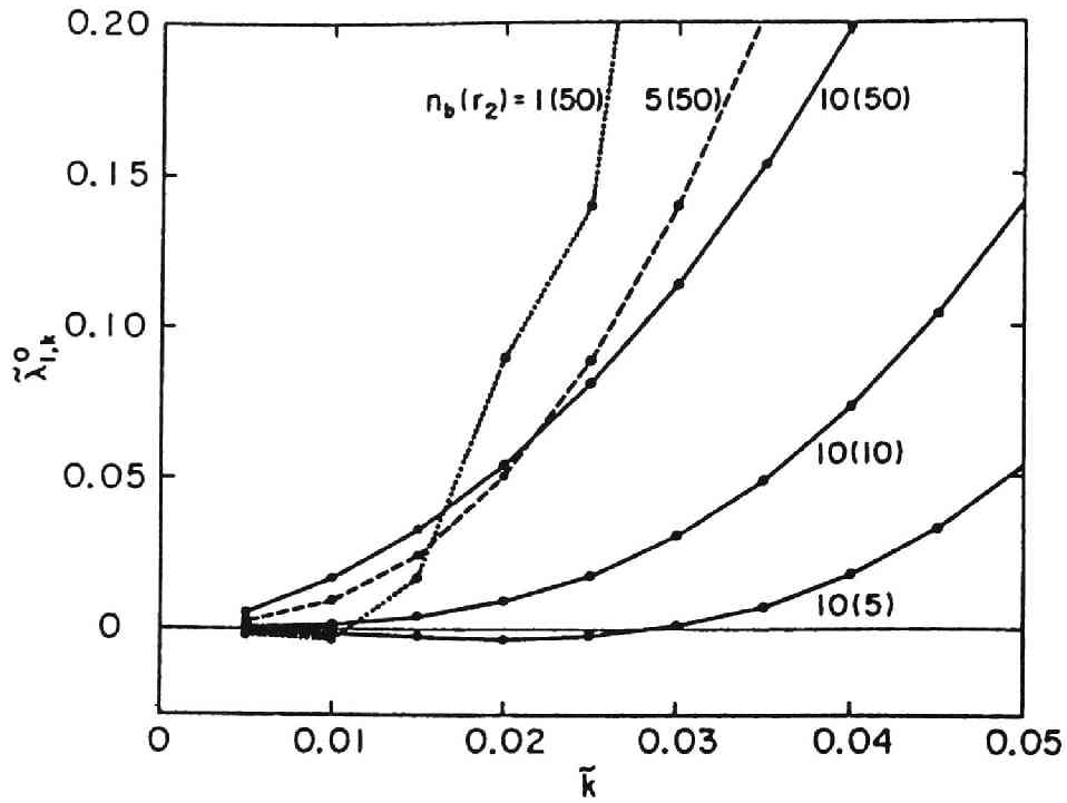
Fig. 4.5. The reduced eigenvalues \tilde{\lambda}_{1,k}^0 plotted against the reduced wave number \tilde{k} for DNA with N=199 and r_1=1 , for the indicated value of n_b and r_2 as n_b(r_2) .
