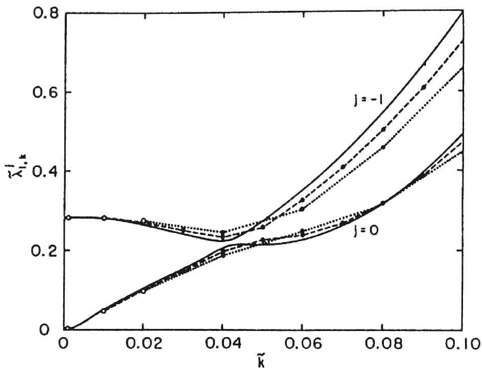
Fig. 4.4. The reduced eigenvalues \tilde{\lambda}_{l,k} plotted against the reduced wave number \tilde{k} for syndiotactic polystyrene with n_b=2 , r_1=1 , and r_2=80 . The full curve represents the values for N=999 , and the broken and dotted line segments connect the values for N=99 and 49, respectively. The open circles represent the values of \tilde{\lambda}_{l,1} .
