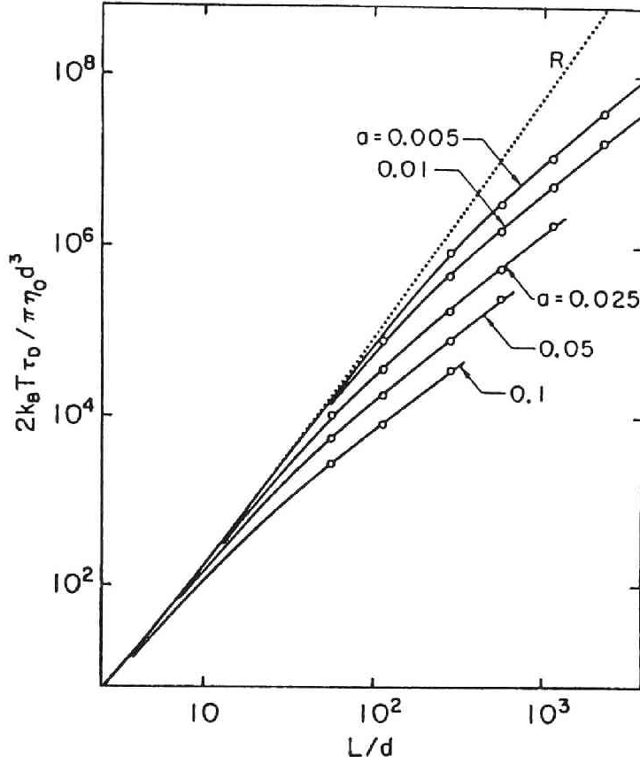
Fig. 4.11. Double logarithmic plots of 2k_B T \tau_D / \pi \eta_0 d^3 against L/d for the KP cylinder ( \kappa_0=0 and \alpha=4=0^\circ ) of contour length L and diameter d . The points represent the original theoretical values. The full curves represent the values calculated from the interpolation formula [Eq. (4.39)] and the dotted curve R those from Eq. (4.40) for the spherocylinder.
