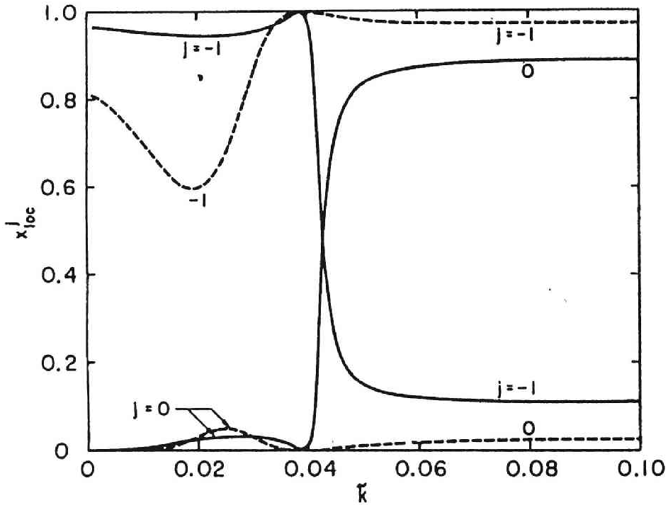
Fig. 4.3. The local mode fractions x_{\text{loc}}^j in the j=0 and -1 branches plotted against the reduced wave number \tilde{k} for syndiotactic polystyrene (full curves) and syndiotactic poly(methyl methacrylate) (broken curves) with the same respective model parameters as in Fig. 4.2.
