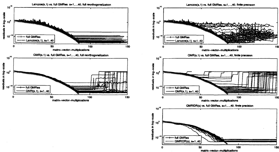
FIG. 3.1. \text{Lanczos}(s, 1) , \text{QMR}(s, 1) , and \text{QMRIDR}(s) versus GMRES: Example based on a random matrix. The shadow vectors are the first vectors of a randomly chosen matrix in \mathbb{R}^{100 \times 40} . The parameter s varies between 1 and 40. The curves of \text{QMRIDR}(s) are tuned by omitting every (s + 1) th step. The GMRES convergence curve is indicated by plus signs, the solid lines are the convergence curves of \text{Lanczos}(s, 1) , \text{QMR}(s, 1) , and \text{QMRIDR}(s) , respectively.
