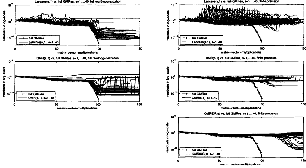
FIG. 3.2. \text{Lanczos}(s,1) , \text{QMR}(s,1) , and \text{QMRIDR}(s) versus GMRES: Example based on a Frank matrix. The shadow vectors are the first vectors of a randomly chosen matrix in \mathbb{R}^{100 \times 40} . The parameter s varies between 1 and 40. The curves of \text{QMRIDR}(s) are tuned by omitting every (s+1) th step. The GMRES convergence curve is indicated by plus signs, the solid lines are the convergence curves of \text{Lanczos}(s,1) , \text{QMR}(s,1) , and \text{QMRIDR}(s) , respectively.
