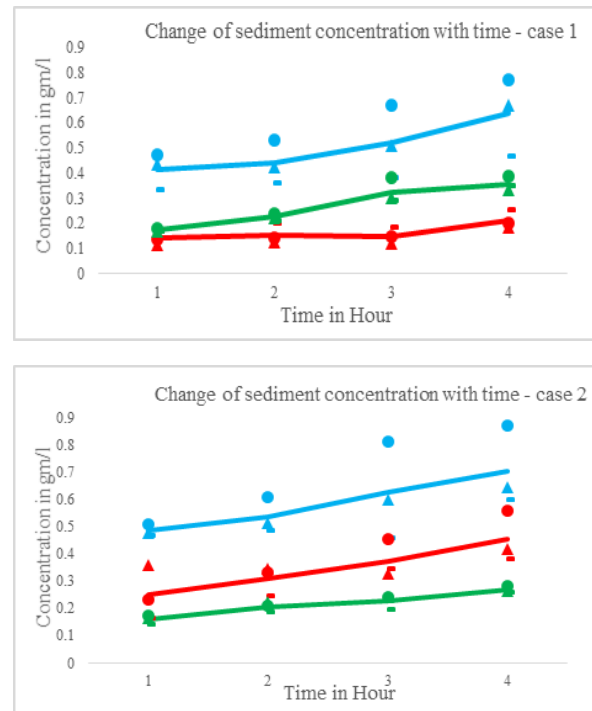
Fig.11 Sediment Concentration at 9 sampling points for case 1 and case 2 (Talchabhadel R. et al, 2016)
