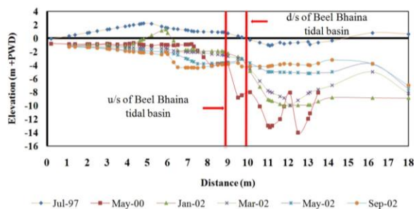
Fig. 6 Temporal variation of profile of Hari River (Khadim F. K. et al, 2013)
