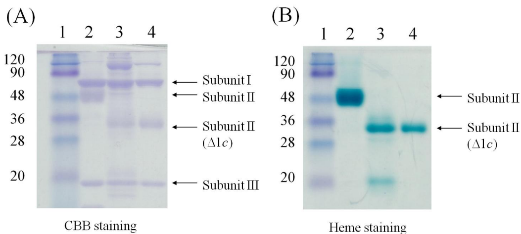
Figure 2. SDS-PAGE photograph of the purified recombinant (native) FDH and variants. heme c moieties in Subunit II are stained by (A) CBB and (B) 3,3',5,5'-tetramethylbenzidine. Lane 1, Molecular mass standard (sizes in kDa are shown on the left); Lane 2, recombinant (native) FDH, Lane 3, \Delta 1c -siteFDH, Lane 4, \Delta 1c FDH.
