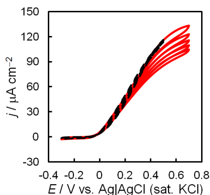
Figure 3. Multi-scan cyclic voltammograms of D-fructose (0.1 M) at an recombinant (native) FDH-adsorbed Au electrode in a McIlvain buffer (pH 4.5) containing 0.1 M D-fructose under anaerobic conditions at a scan rate of 10 \text{ mV s}^{-1} . The broken line indicates a multi-can cyclic voltammogram in the potential range from -0.3 \text{ V} to 0.5 \text{ V} .
