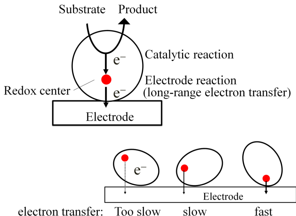
Figure 1. Schemes of (A) a model of the direct electron transfer pathway and (B) the effects of the adsorption orientation of enzymes on the distance between the electrode surface and the redox active site and the interfacial electron transfer rate constant.
