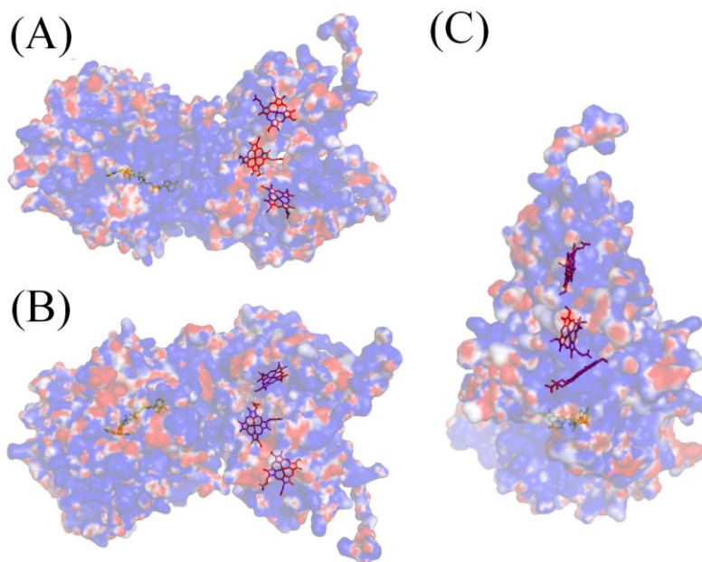
Figure 5. (A): Electrostatic characteristics of the protein surface of FDH. Positive potentials are drawn in blue, negative potentials in red. Heme 1c, 3c, and 2c locate from the top to bottom. (B): After rotation around the horizontal axis by 180° from (A). (C): After rotation around the vertical axis by 90° from (A).
