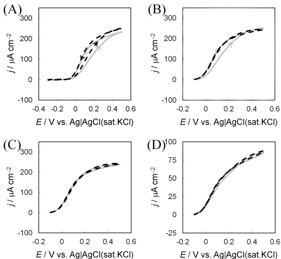
Figure 4. CVs of D-fructose oxidation at M450Q \Delta 1cFDH-adsorbed Au electrodes in McB (pH 4.5) in the presence of 0.2 M D-fructose under anaerobic conditions at \nu = 10 \text{ mV s}^{-1} . (A) CV in scanning from -0.3 \text{ V} after adsorption of the variant at the open circuit potential. The gray line is the first scan, and the dashed black line is the second scan. (B) CV in scanning from -0.1 \text{ V} . The other conditions are identical with those of (A). (C) CV after adsorption of the variant at 0.5 \text{ V} . The other conditions are identical with those of (B). (D) CV after the following treatments: the variant was adsorbed at the open circuit potential, and the potential was scanned 2 cycles from -0.1 \text{ V} to 0.5 \text{ V} . Thereafter, the electrode was held at -0.3 \text{ V} for 5 min, and then transferred to a fresh electrochemical solution (McB, pH 4.5) containing 0.2 M D-fructose.
