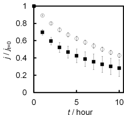
Figure 4. Stability during the continuous operation of the recombinant (native) FDH (open circles) or \Delta 1c FDH (closed squares) adsorbed on electrodes at 0.5 V in McB (pH 4.5) and in the presence of 100 mM D-fructose under anaerobic conditions. The error bars were evaluated using Student's t -distribution at a 90% confidence level in three repeated experiments.
