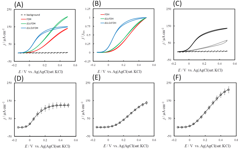
Figure 3. (A) Original CVs and (B) normalized CVs of D-fructose oxidation at the recombinant (native) FDH-, \Delta 1c FDH-, and \Delta 1c2c FDH-adsorbed electrodes in McB (pH 4.5) in the presence of 100 mM D-fructose under anaerobic conditions at \nu = 10 \text{ mV s}^{-1} . The broken line in panel (A) indicates the background current at the bare Au electrode. In panel (B), the background current was subtracted. In panel (C), the solid line is the CV at the \Delta 1c2c FDH-adsorbed electrode in McB (pH 4.5) in the presence of 100 mM D-fructose under anaerobic conditions; the broken line is background, and the dotted line is a CV after the addition of KCN (1 mM in final concentration) at \nu = 10 \text{ mV s}^{-1} . Panels (D) to (F) show fitted curves obtained by non-linear least square method. The circles are the waves of the forward scan measured with (D) the \Delta 1c2c FDH-, (E) recombinant (native) FDH-, and (F) \Delta 1c FDH-adsorbed electrodes. The insets indicate the evaluated parameters. The error bars were evaluated by the Student t -distribution at a 90% confidence level.
