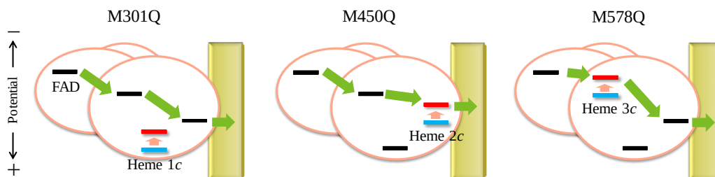
Figure 4. Cartoons of electron transfer in the three mutants
