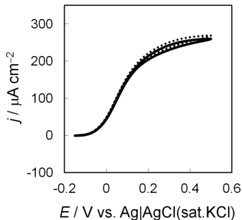
Figure 2. (A): CVs D-fructose oxidation at M450Q \Delta 1cFDH-adsorbed Au electrodes in McB (pH4.5) in the presence of 0.2 M D-fructose under anaerobic conditions at v = 10 \text{ mV s}^{-1} in quiet solution (black solid line) and under convective conditions at \omega = 2000 \text{ rpm} (black dotted line).
