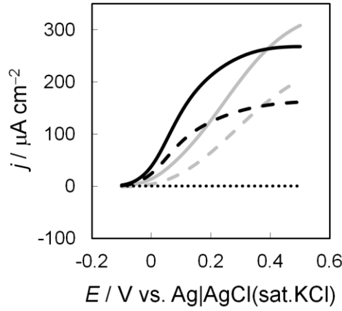
Figure 3. Linear sweep voltammogram of D-fructose oxidation at the recombinant (native) FDH- (dashed gray line), M450QFDH- (dashed black line), \Delta 1 cFDH- (gray line) and M450Q \Delta 1 cFDH- (black line) adsorbed electrodes in McB (pH4.5) in the presence of 0.2 M D-fructose under anaerobic conditions. The scan rate was 10 \text{ mV s}^{-1} . The dotted line indicates the background at the bare Au electrode.
