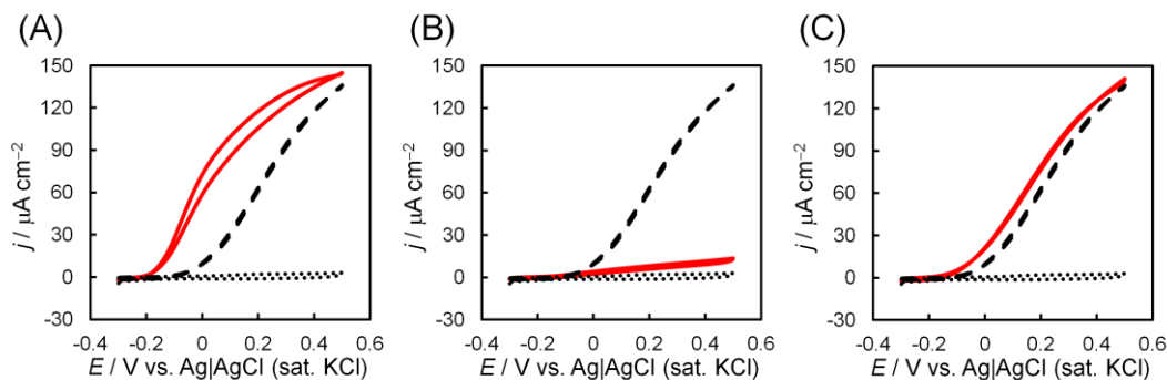
Figure 2. Cyclic voltammograms of D-fructose oxidation at (A-C: broken line) a recombinant (native) FDH-adsorbed Au electrode and (solid lines) (A) M450Q, (B) M578Q, and (C) M301Q mutant adsorbed Au electrodes in a McIlvain buffer (pH 4.5) containing 0.1 M D-fructose under anaerobic conditions at a scan rate of 10 \text{ mV s}^{-1} . The dotted lines indicate a background voltammogram at a bare Au electrode.
