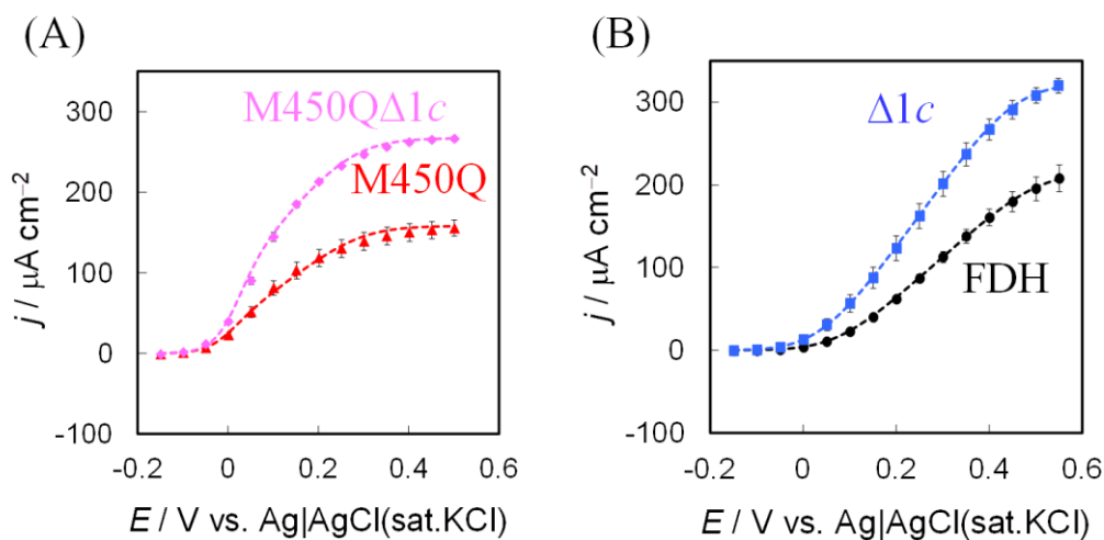
Figure 9. Steady-state voltammograms of D-fructose oxidation at (A) M450QΔ1cFDH- (pink diamond) and M450QFDH- (red triangle) adsorbed electrode and (B) Δ1cFDH- (blue square) and the recombinant (native) FDH- (black circle) adsorbed electrodes in McB (pH4.5) in the presence of 0.2 M D-fructose under anaerobic conditions. The scan rate was 10 \text{ mV s}^{-1} . The error bars were evaluated by the Student t -distribution at a 90% confidence. Each dashed line indicates the regression result estimated according to Eqs. (1) and (2).
