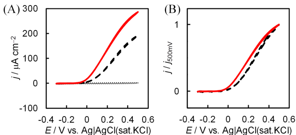
Figure 3. CVs (A) and normalized CVs (B) of D-fructose oxidation at the recombinant (native) FDH- (broken line) or the \Delta 1c FDH- (solid line) adsorbed electrodes in McB (pH 4.5) in the presence of 100 mM D-fructose under anaerobic conditions. The scan rate was 10 \text{ mV s}^{-1} . The dotted line indicates the background at the bare Au electrode.
