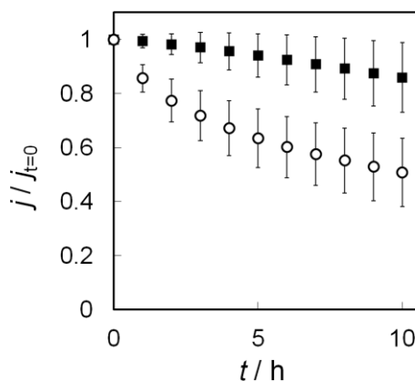
Figure 8. Stability of the recombinant (native) FDH (closed squares) and M450QΔ1cFDH (open circles) adsorbed on bare Au electrodes at 25 °C in McB (pH 4.5) in the presence of 0.2 M D-fructose. The normalized values of j_{\text{lim}} obtained from the second cycle CVs taken every
