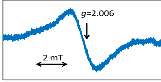
Figure 4. ESR spectrum of D-fructose-reduced state of \Delta 1c2cFDH at pH 6.0
