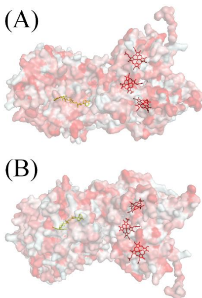
Figure 6. (A): Surface hydrophobicity of FDH. Hydrophobic residues are highlighted in red, hydrophilic in white. Heme 1c, 3c, and 2c locate from the top to bottom. (B): After rotation around the horizontal axis by 180° from (A). This crystal structure model does not have CHR because the template protein does not have CHR. However, CHR seems not to play significant role in DET-type bioelectrocatalysis, because \Delta\text{chrFDH} (lacking CHR) show clear DET-type catalytic wave according to previous research.
