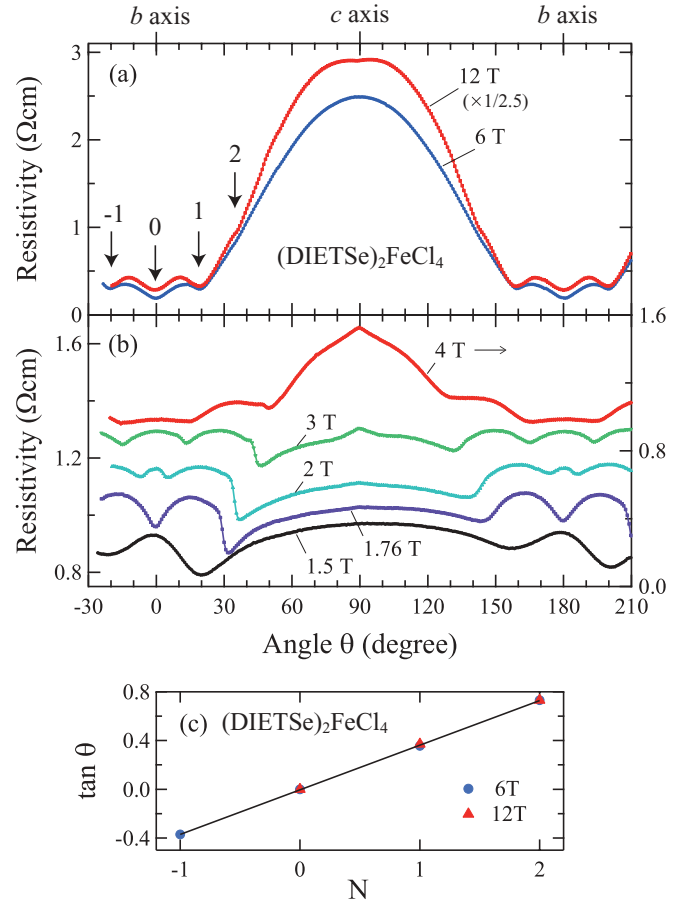
FIG. 7. (Color online) Angular dependence of MR in (\text{DIETSe})_2\text{FeCl}_4 at 1.5 K under 6.5 kbar in the high magnetic field region (a) and the low magnetic field region (b). (c) The positions of the dips in the MR at 6 T and 12 T plotted against \tan \theta .
