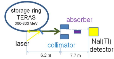
Fig. 2. Schematic drawing of the experimental set-up.
