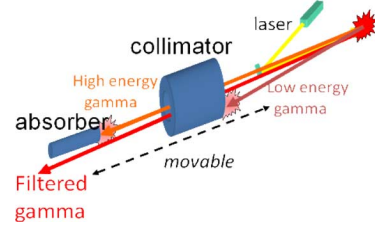
Fig. 1. Principle of the absorber-collimator method.
