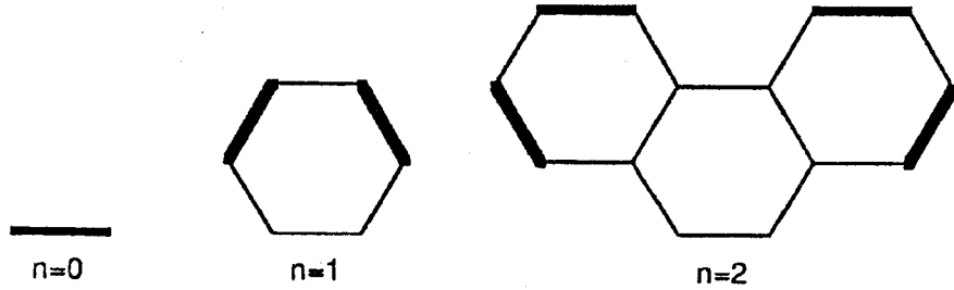
Figure 15: The surface of the n -th generation of a generalized cactus tree.
