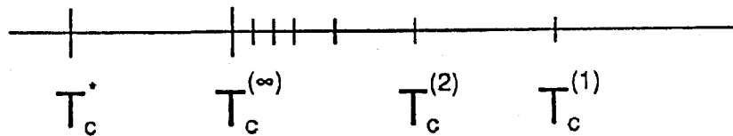
Figure 4: The series [5] of the critical points \{T_c^{(n)}\} of the cactus trees connected at each boundary site as shown in Fig. 3.
