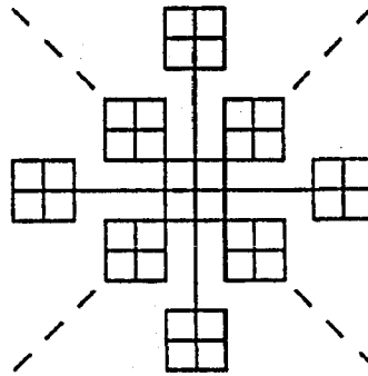
Figure 3: A cactus tree connected at each boundary site [5].
