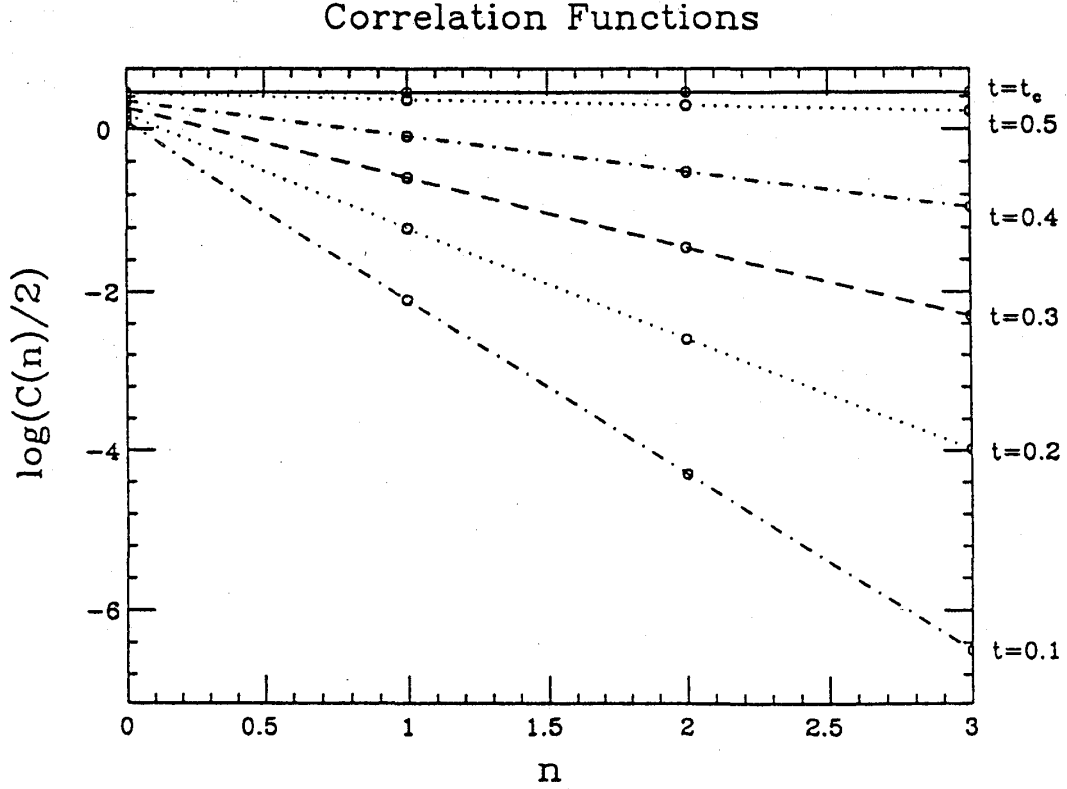
Figure 16: Correlation functions in some temperatures, where t = \tanh \beta J .
