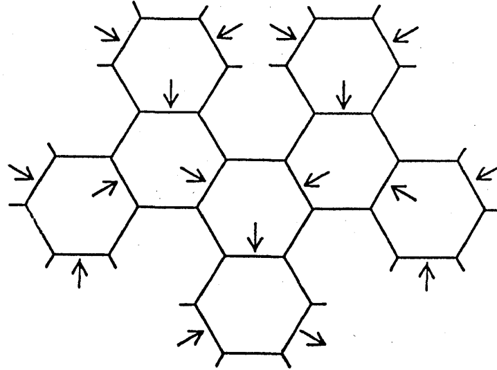
Figure 8: A generalized honeycomb cactus tree [5].
