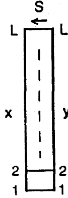
Figure 6: Transfer-matrix in the two-dimensional square lattice.
