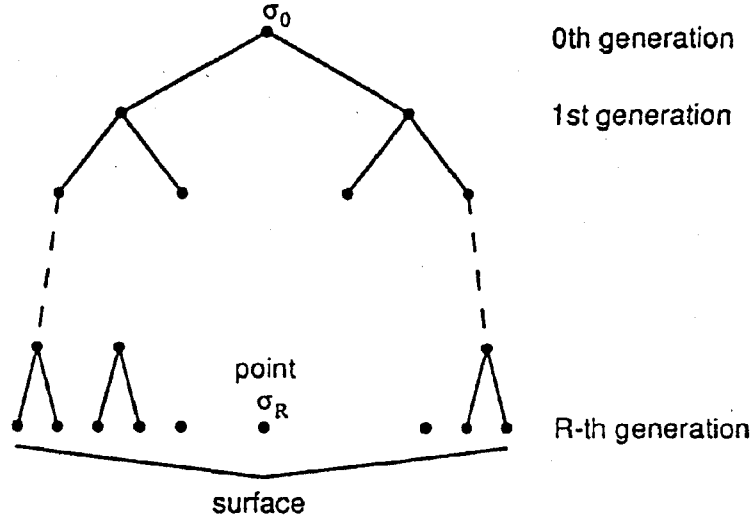
Figure 14: 0 to R -th generation spins.
