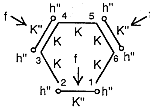
Figure 9: A honeycomb cactus cell.
