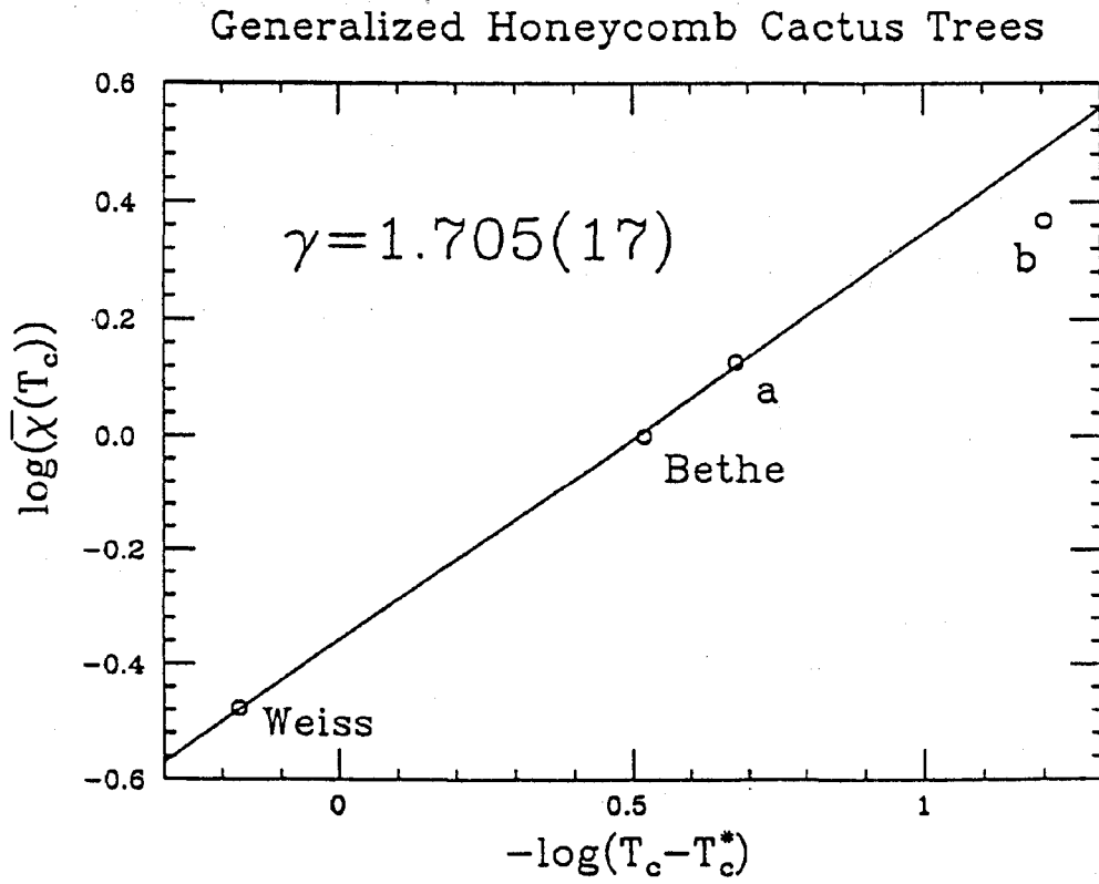
Figure 11: The data points, "Weiss", "Bethe" and "a", are fitting to the function (5.19).
