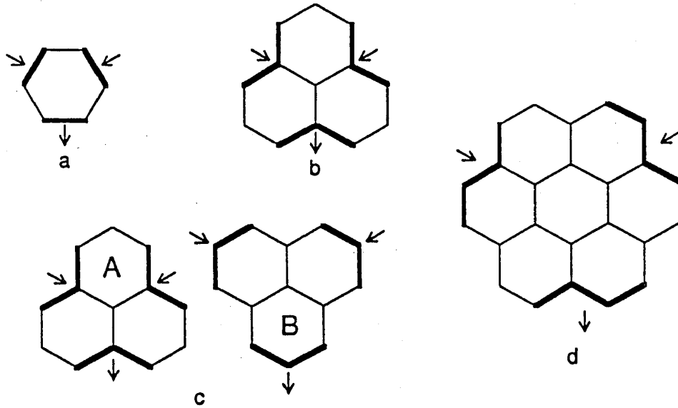
Figure 10: Unit cells of treated models.
