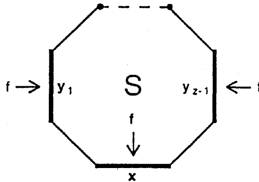
Figure 7: A general cactus cell with z connection-lines and the corresponding confluent transfer-matrix S [5].
