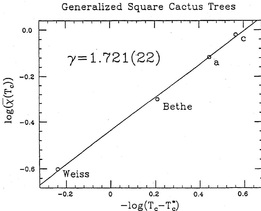
Figure 13: The data points, "Weiss", "Bethe", "a" and "c", are fitting to the function (5.19).
