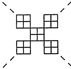
Figure 2: A square cactus tree [5].
