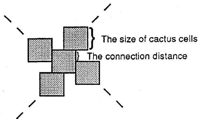
Figure 5: A generalized square cactus tree [5].
