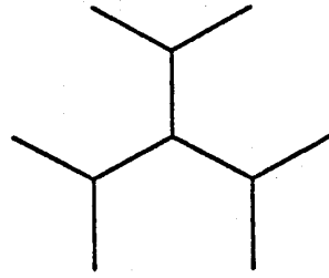
Figure 1: A Cayley tree ( z = 3 ).
