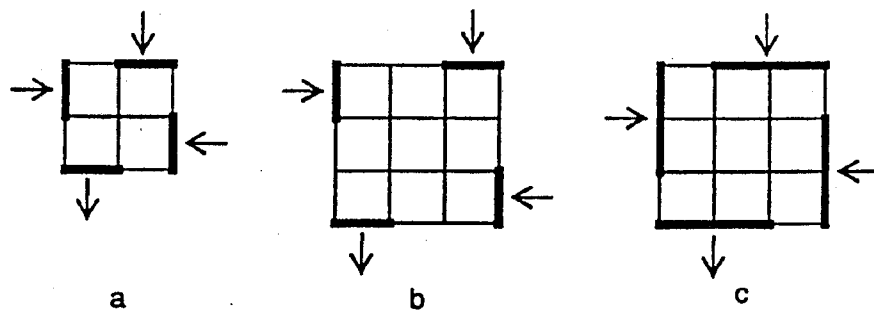
Figure 12: Unit cells of treated models.
