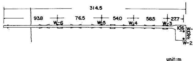
Fig. 7 Position of wave gauges at pier.
