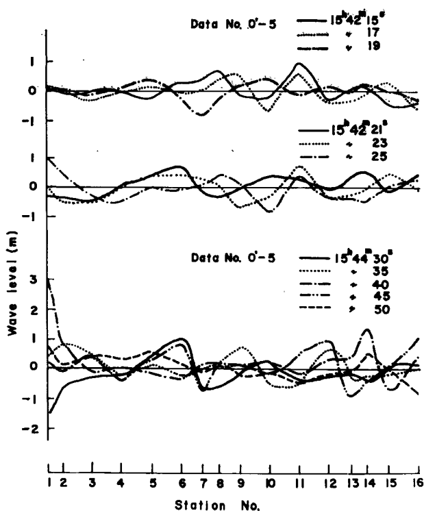
Fig. 12 Wave profiles.
