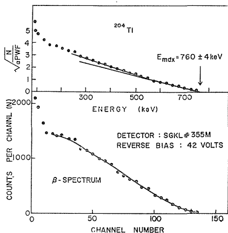
Fig. 11. Beta-ray spectrum of ^{204}\text{Tl} and its Fermi plot observed with a p-i-n silicon junction detector at room temperature.
