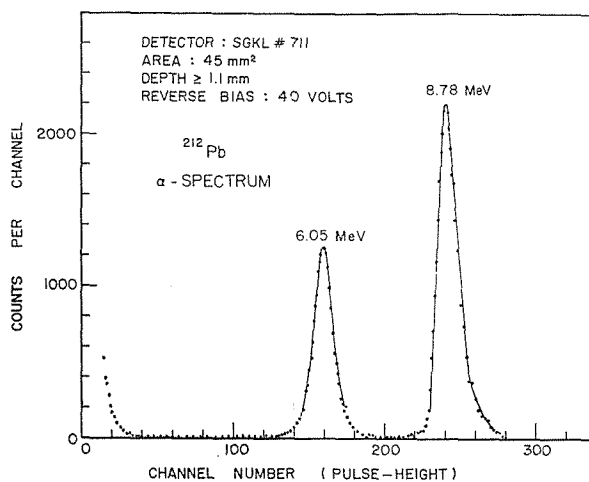
Fig. 2. Alpha particle spectrum from ^{212}\text{Pb} .
