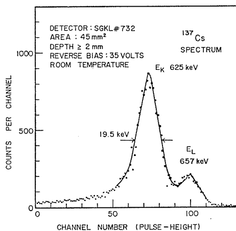
Fig. 7. Pulse-height spectrum of conversion electrons of ^{137}\text{Ba} observed with a p-i-n silicon junction detector at room temperature.
