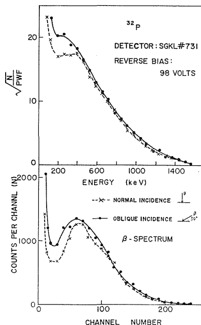
Fig. 14. Beta-ray spectrum of ^{32}\text{P} and its Fermi plot observed with a p-i-n silicon junction detector at room temperature.
