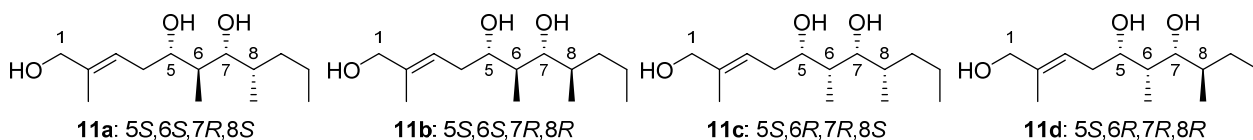
Figure 2. Possible triols obtained by LiAlH 4 -mediated degradation of 1 .
