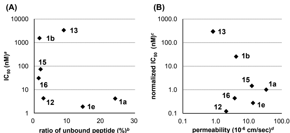
Figure 7. The relationships between physicochemical properties and cytotoxicity. (A) Scatter plot between ratio of unbound peptide and cytotoxicity IC 50 . (B) Scatter plot between normalized IC 50 and membrane permeability. a IC 50 values are the concentrations for 50% growth inhibition of A549 cells. b Ratio of unbound peptide was evaluated in medium supplemented with 10% (v/v) fetal bovine serum. c Normalized IC 50 = IC 50 × unbound peptide ratio; d Membrane permeability was evaluated by PAMPA (pH = 7.4).
