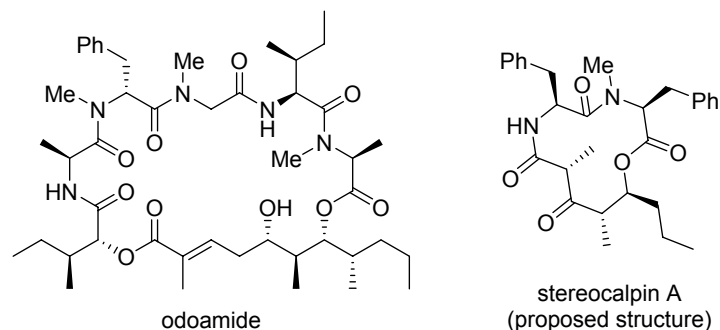
Figure 7. Synthetic targets in this thesis.
