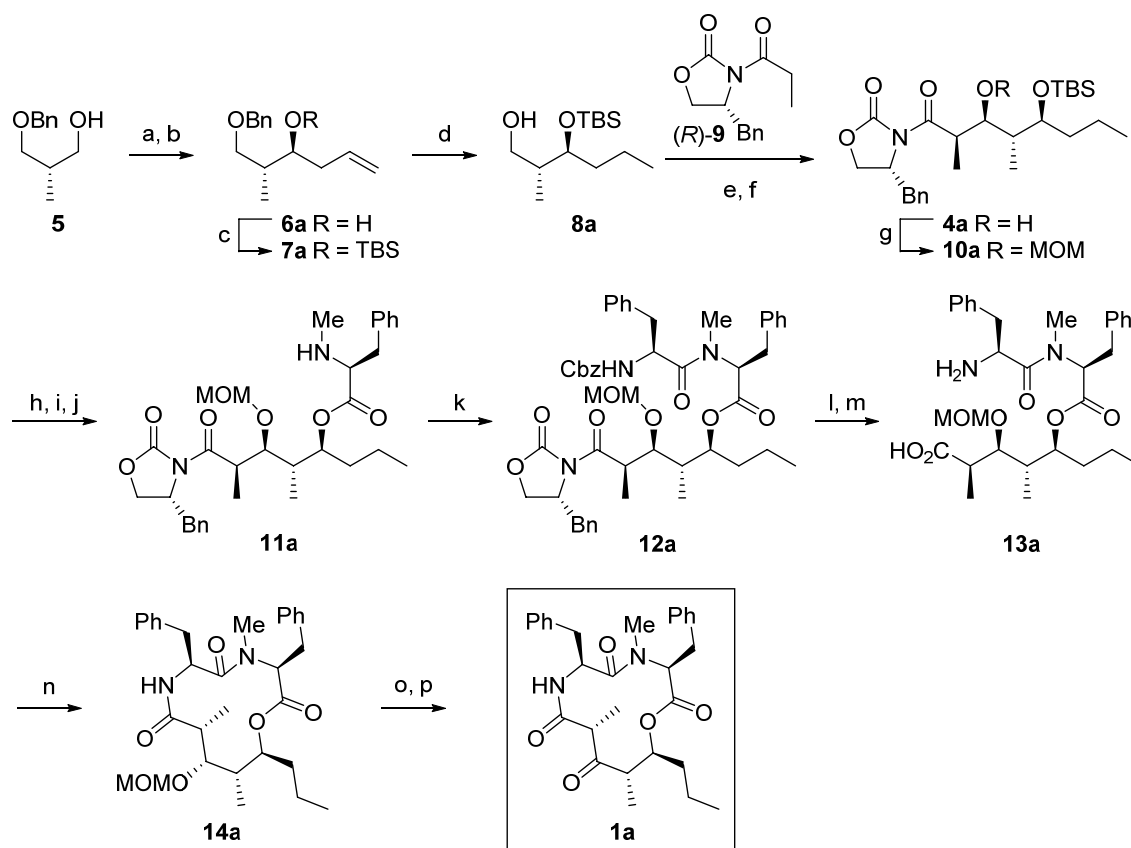
Scheme 1. Synthesis of the proposed structure of stereocalpin A ( 1a ). Reagents and conditions: (a) (COCl) 2 , DMSO, ( i -Pr) 2 NEt, CH 2 Cl 2 , -78 °C to 0 °C; (b) allyltributylstannane, SnCl 4 , CH 2 Cl 2 , -78 °C, 80% (2 steps, dr 15:1); (c) TBSCl, imidazole, DMF, 0 °C to rt, 91%; (d) Pd/C, H 2 , EtOH, rt, 87%; (e) (COCl) 2 , DMSO, ( i -Pr) 2 NEt, CH 2 Cl 2 , -78 °C to 0 °C; (f) ( R )- 9 , n -Bu 2 BOTf, ( i -Pr) 2 NEt, CH 2 Cl 2 , -78 °C to -10 °C, 86% (2 steps); (g) MOMCl, ( i -Pr) 2 NEt, 1,2-dichloroethane, rt to 40 °C, 93%; (h) HF·pyridine, THF, pyridine, 0 °C to rt; (i) Fmoc-L-MePhe-OH, EDCI·HCl, DMAP, CH 2 Cl 2 , 0 °C; (j) Et 2 NH, MeCN, rt, 82% (3 steps); (k) Cbz-L-Phe-OH, HATU, ( i -Pr) 2 NEt, CH 2 Cl 2 , 0 °C to rt, 91%; (l) LiOH, H 2 O 2 , THF, H 2 O, 0 °C to rt; (m) Pd/C, H 2 , MeOH, rt; (n) HATU, HOAt, ( i -Pr) 2 NEt, DMF, rt, 54% (3 steps); (o) HCl, MeOH, H 2 O, 0 °C to 40 °C; (p) Dess-Martin periodinane, CH 2 Cl 2 , rt to 40 °C, 78% (2 steps).
