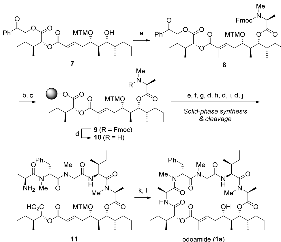
Scheme 1. Synthesis of odoamide ( 1a ) via solid-phase peptide synthesis. Reagents and conditions: (a) Fmoc-L-MeAla-Cl, ( i -Pr) 2 NEt, 1,2-dichloroethane, 40 °C; (b) Zn, AcOH, rt; (c) Cl-(2-Cl)Trt resin, ( i -Pr) 2 NEt, CH 2 Cl 2 , rt; (d) 20% piperidine/DMF, rt; (e) Alloc-L-Ile-OH, DIC, HOAt, DMF, rt; (f) Pd(PPh 3 ) 4 , PhSiH 3 , CH 2 Cl 2 , rt; (g) Fmoc-Sar-OH, HOBt·H 2 O, DIC, DMF, rt; (h) Fmoc-D-MePhe-OH, HATU, ( i -Pr) 2 NEt, DMF, rt; (i) Fmoc-L-Ala-OH, HATU, ( i -Pr) 2 NEt, DMF, rt; (j) 30% HFIP/CH 2 Cl 2 , rt; (k) HATU, HOAt, collidine, DMF, rt; (l) AgNO 3 , 2,6-lutidine, THF, H 2 O, rt to 70 °C.
