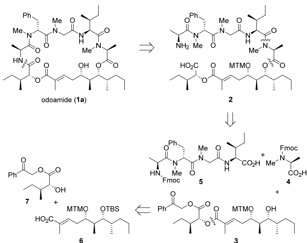
Scheme 1. Retrosynthetic analysis of odoamide ( 1 ).
